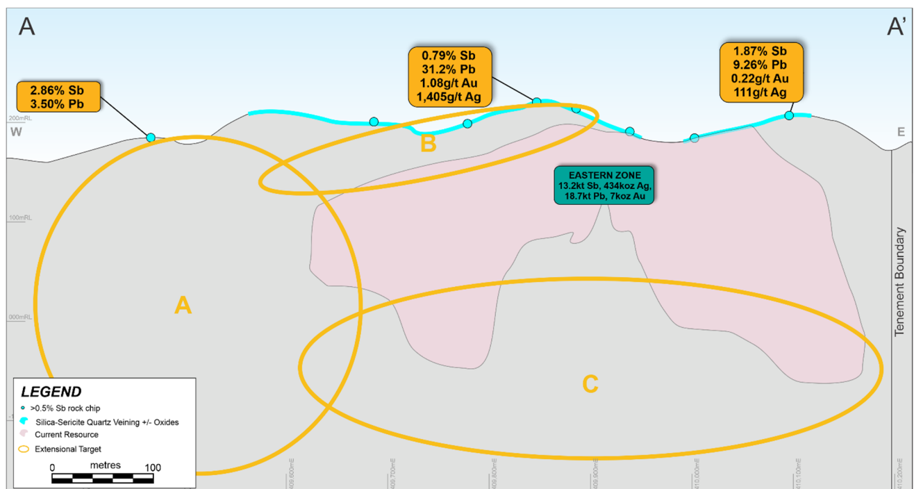
Figure 2: Schematic long section through the Eastern Zone of Mt Clement showing the Str1 Resource and areas targeted for extension and upgrade drilling.
