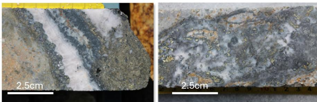
Figure 2. Quartz-sphalerite-pyrite vein at 14.15m (GT002: 0.3g/t Au and 1.2% Zn from 14m), Figure 3. chalcopyrite-sphalerite-quartz vein at 18.9m (GT005: 2.8g/t Au, 0.6% Cu and 1% Zn from 18m)
