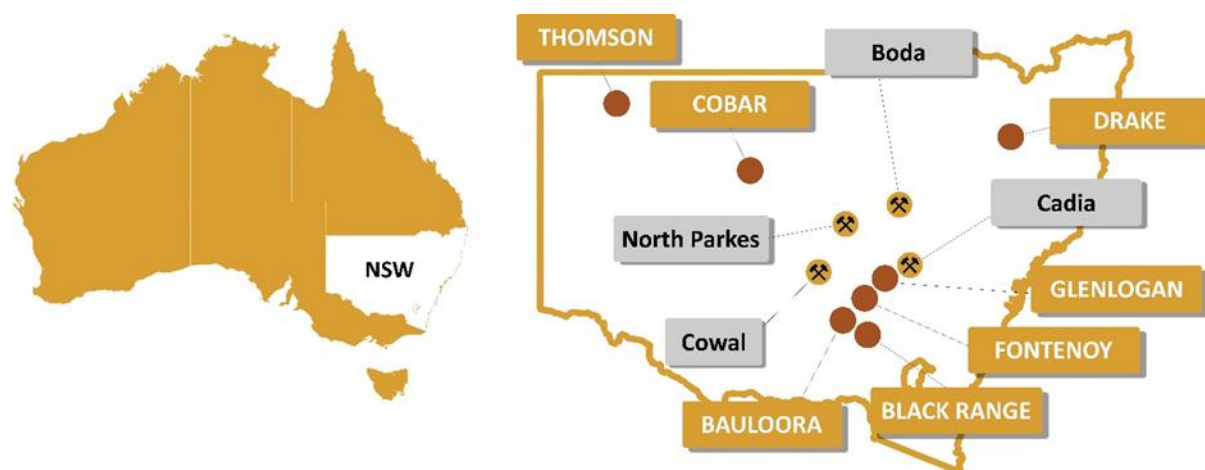
Figure 8. Location of Legacy Minerals' Projects in NSW, Australia, and major mines and deposits
