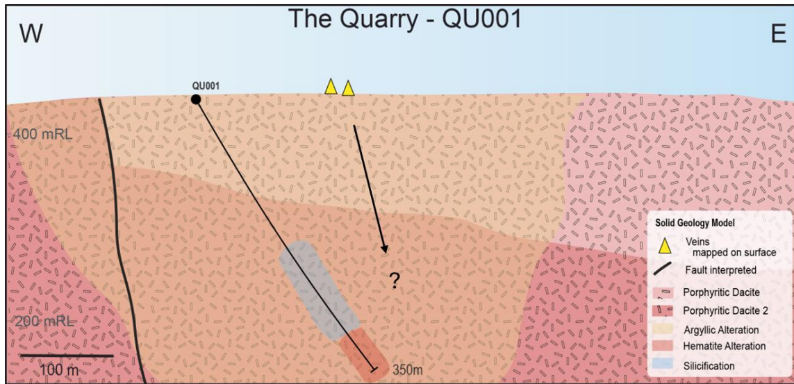
Figure 3. QU001 cross section (MGA94z55 6177903mN) showing solid geology interpretation.
