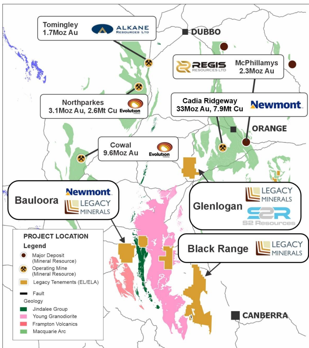
Figure 7. Regional setting of the Bauloora Project and major deposits in NSW v
