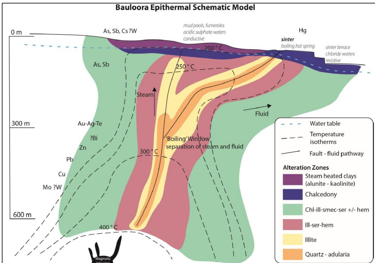
Figure 4. Bauloora epithermal schematic model showing zone alteration patterns (modified from Buchanan 1981, Morrison et. al 1995).
