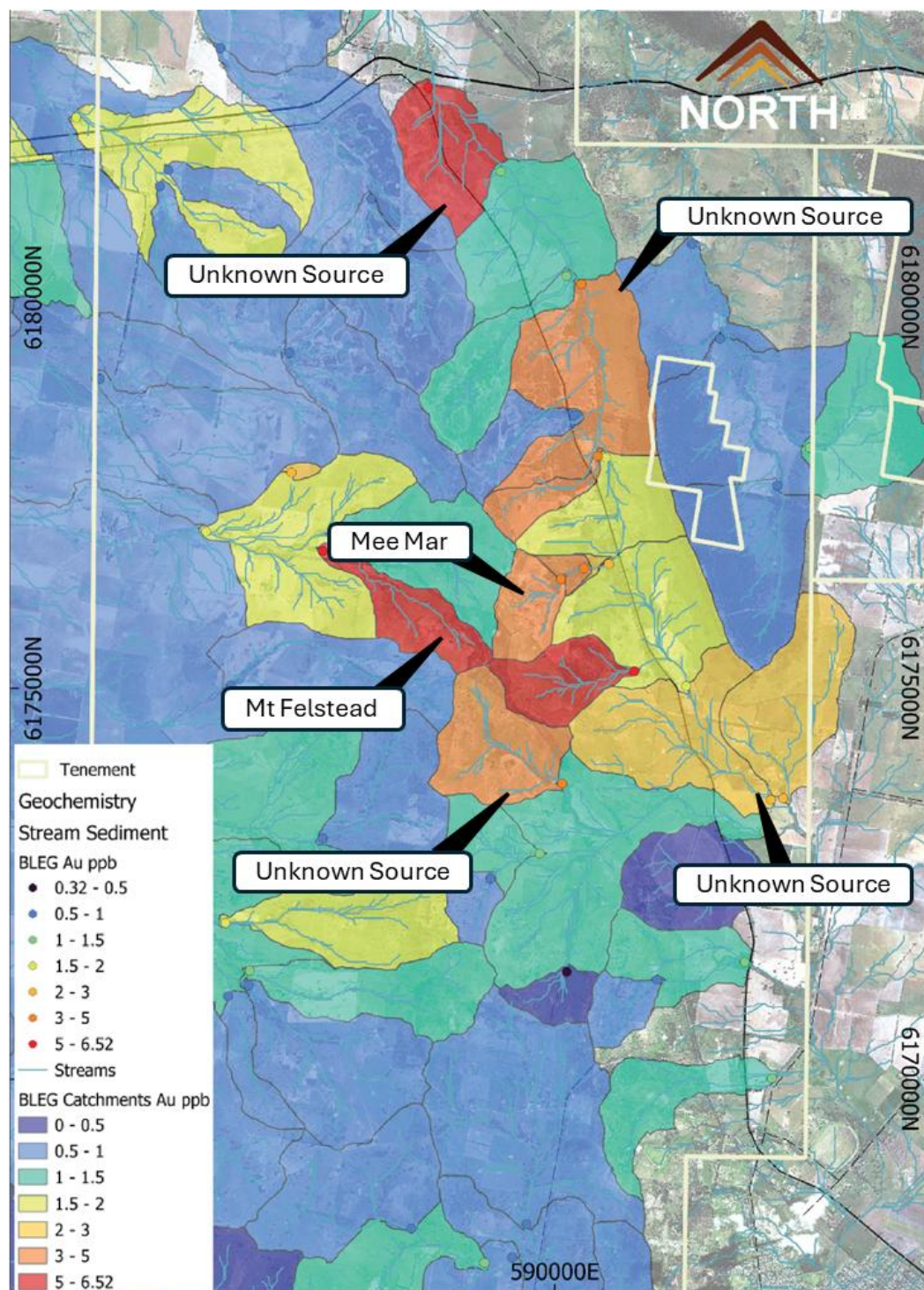
Figure 5. Bauloora Project overview showing BLEG sampling locations and anomalous drainage areas warranting follow up work.
