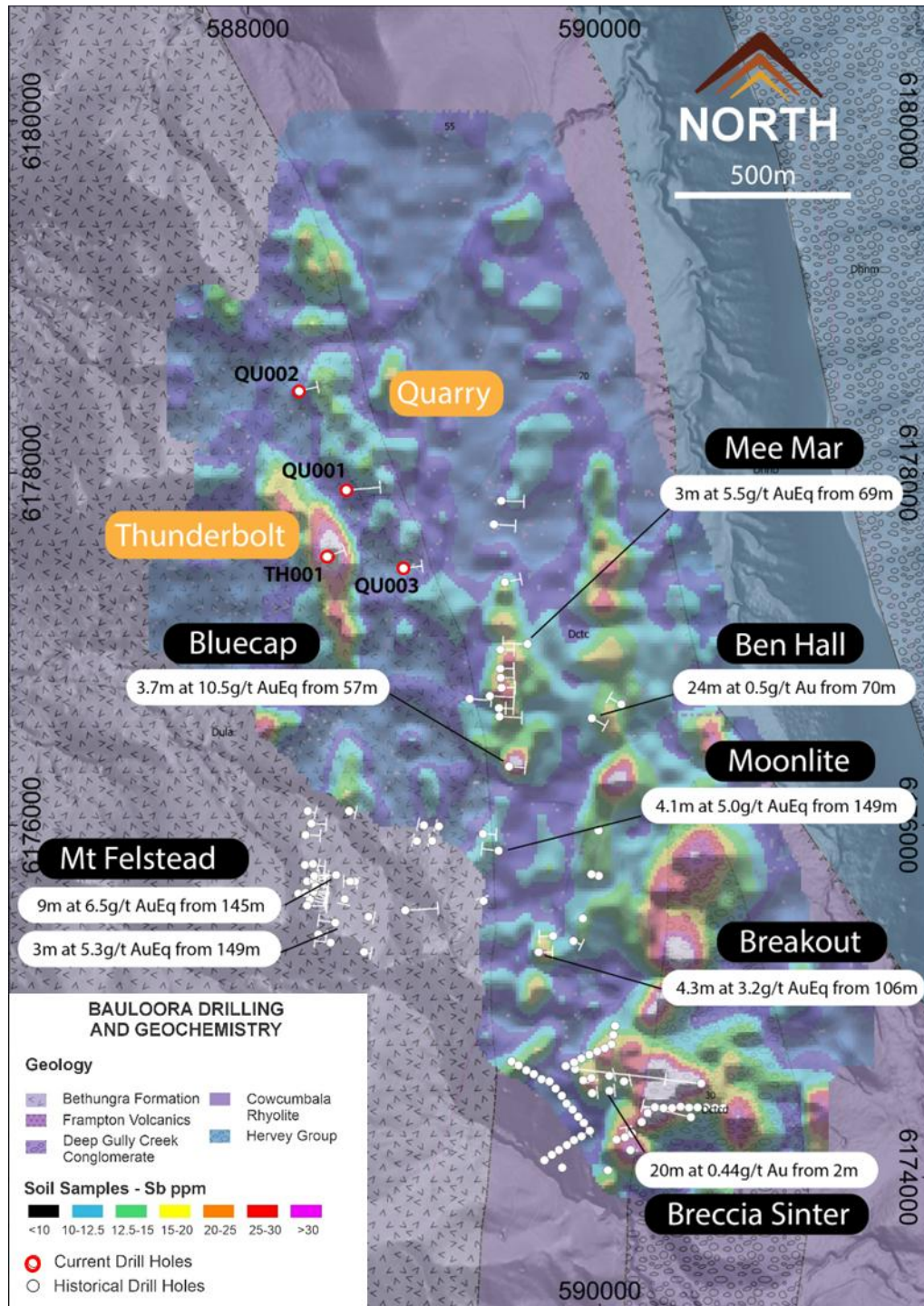
Figure 1: Bauloora Project with recently completed drilling (red border) and previous highlight drilling results over Sb in soil sampling and regional geology interpretation.
