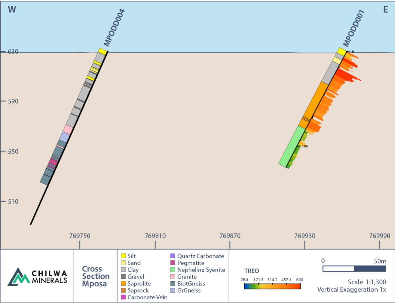
Figure 6: Cross section
