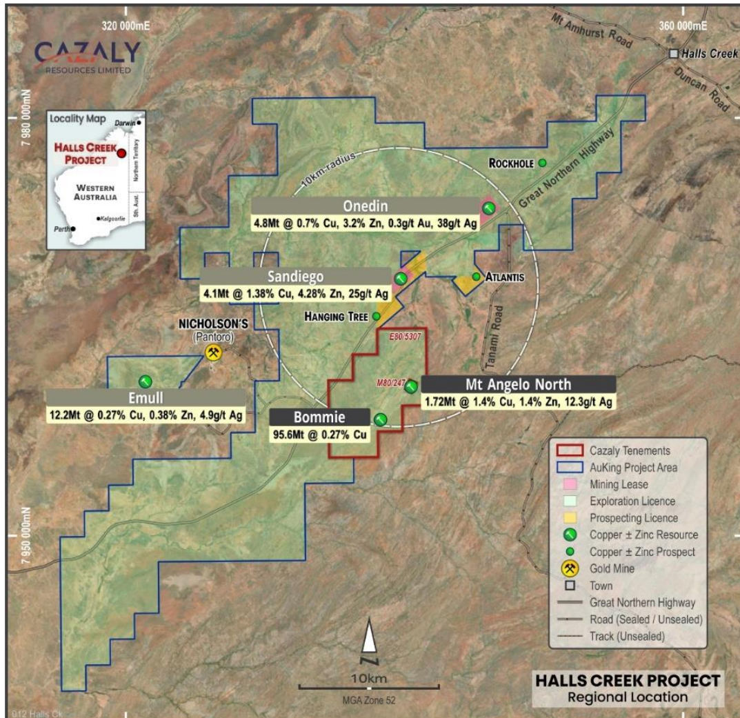
Figure 4. Halls Creek Copper Project with mineral resource locations relative to AuKing's project area.
