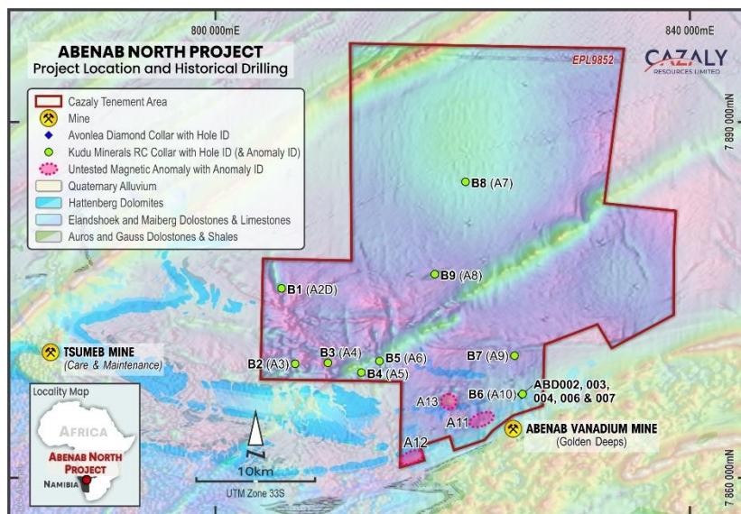
Figure 3. Abenab North Project with historical drilling and untested magnetic anomalies.
