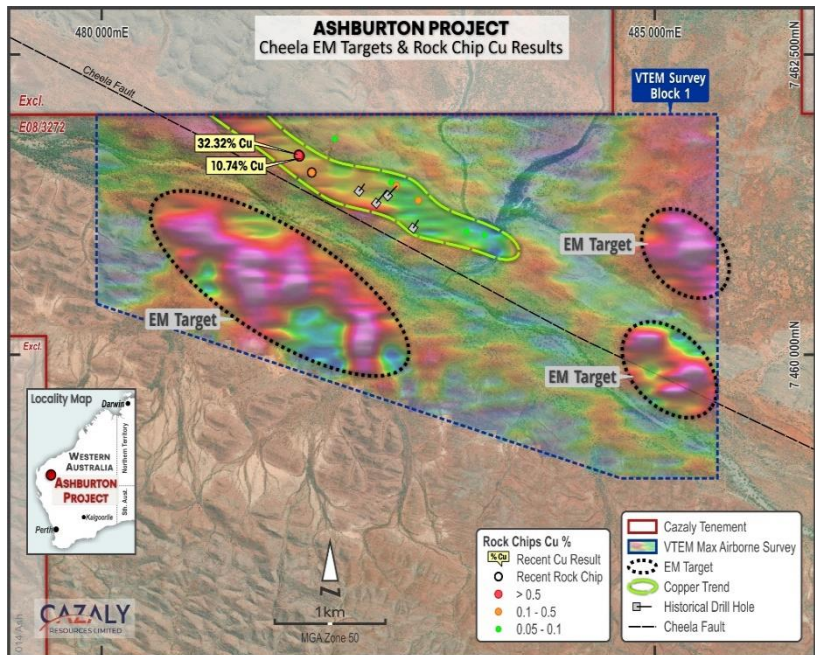
Figure 5. Location of the Ashburton project with priority EM targets and rock chip results at the Cheela Prospect.
