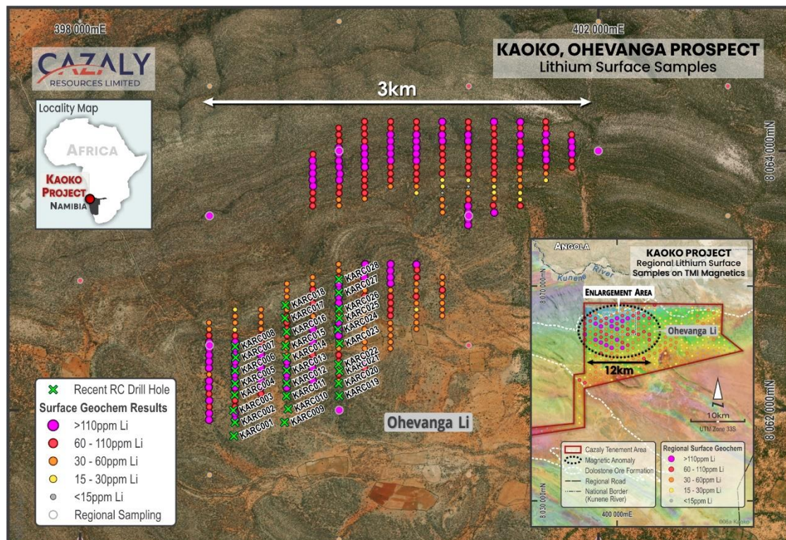
Figure 2. Location of the Ohevanga lithium anomaly and the high priority Phase 1 drill target
