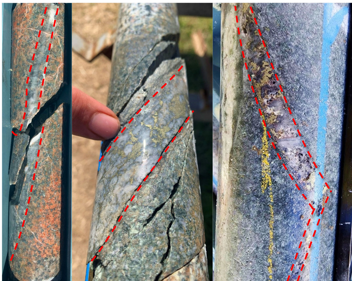
Figure 4. Left to Right. MRDD001, 227.3m strong potassic alteration of granodiorite with sulphide bearing quartz-vein (0.6m @ 10ppb Au, 0.5g/t Ag & 857ppm Cu). MRDD002, 136.15m quartz-sulphide vein within shear of strong sericite alteration of granodiorite (0.5m @ 5.89g/t Au, 21.1g/t Ag & 0.7% Cu). MRDD003, 34.9m strong silica and sericite alteration in granodiorite, quartz veins with visible chalcopyrite (0.6m @ 0.3g/t Au, 37g/t Ag & 1.6% Cu).
