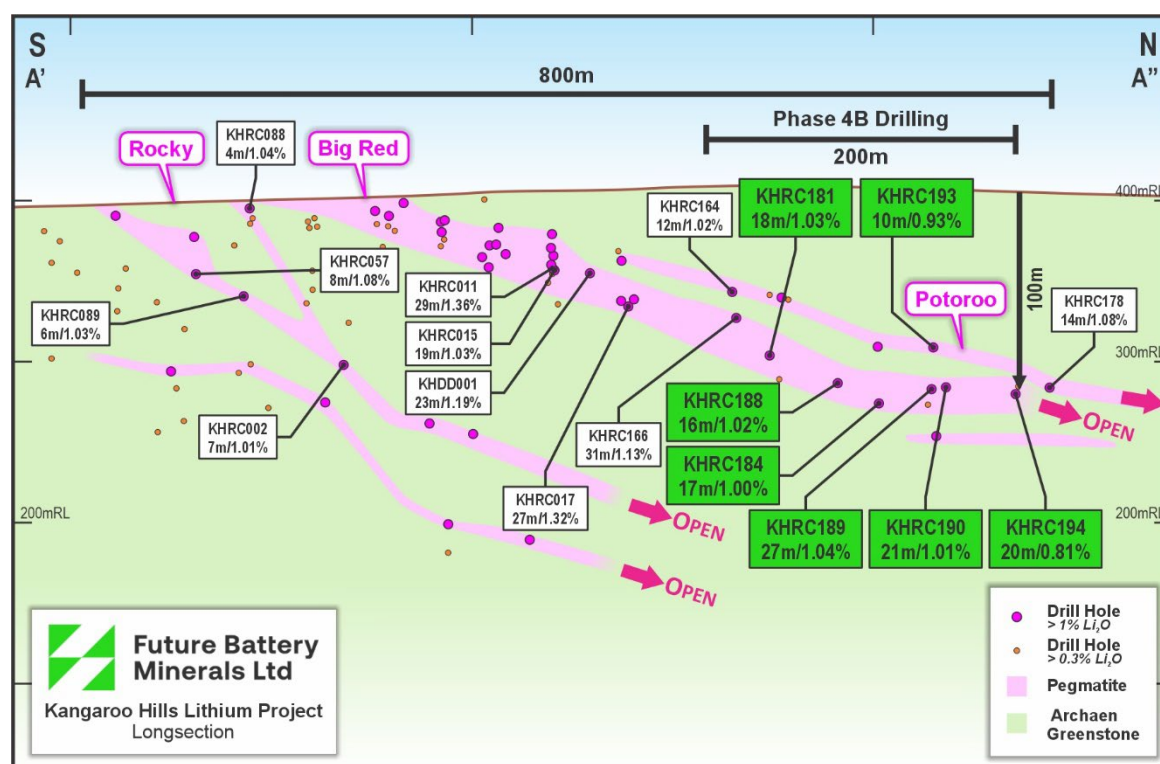
Figure 3. Phase 4B KHLPL schematic long section
