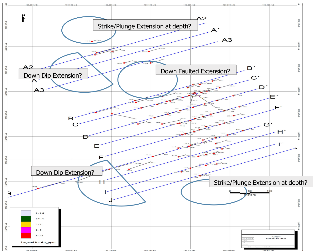
Figure 2: Exploration Targets
