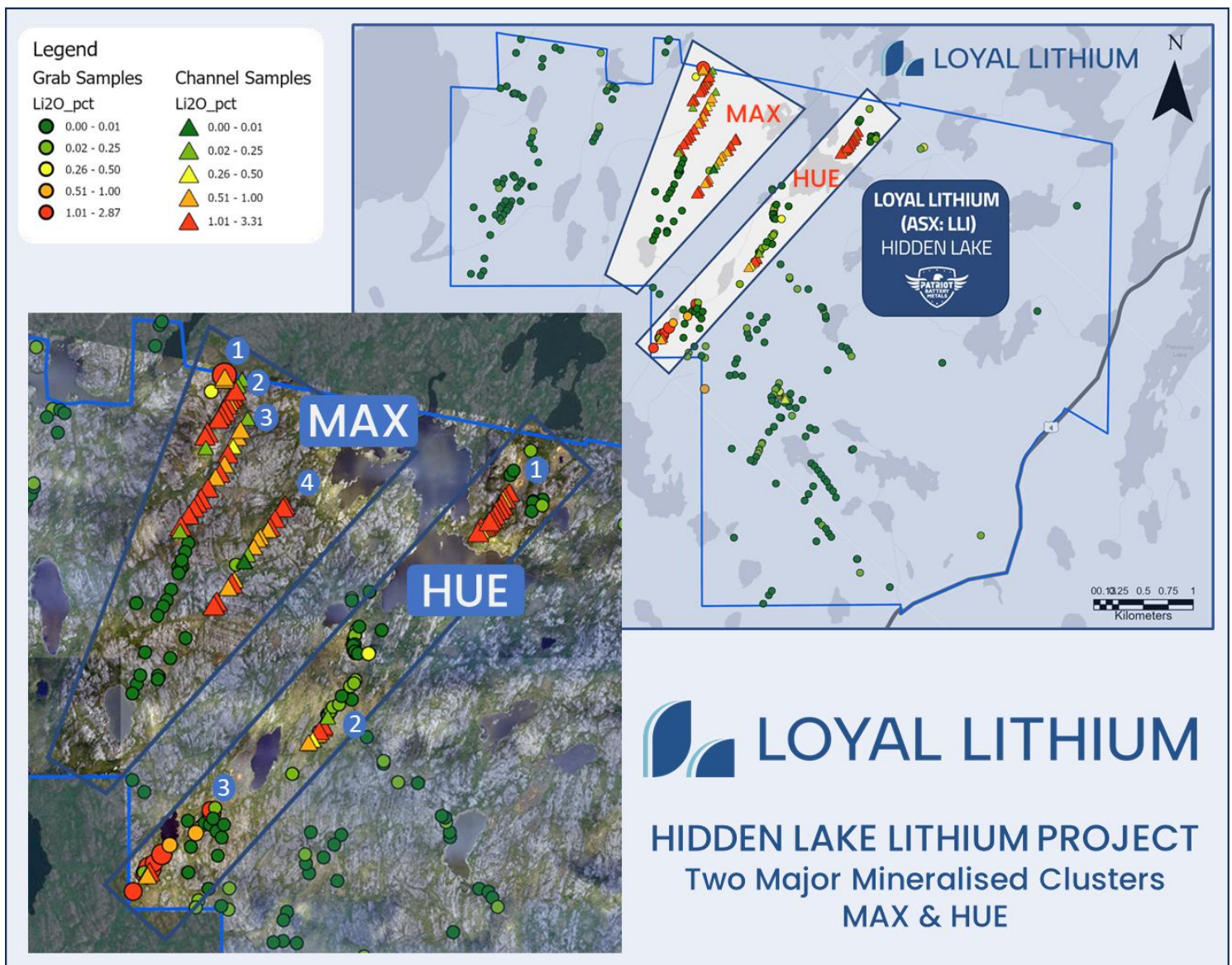
Hidden Lake Lithium Project: Seven spodumene mineralised clusters of dykes (Max 1 – 4 & Hue 1 – 3).
