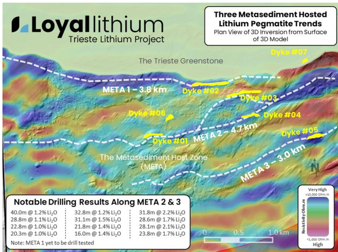
Trieste Lithium Project: Three Metasediment Hosted Lithium Pegmatite Trends – Plan view from surface of 3D model (6, 7, 8) .
