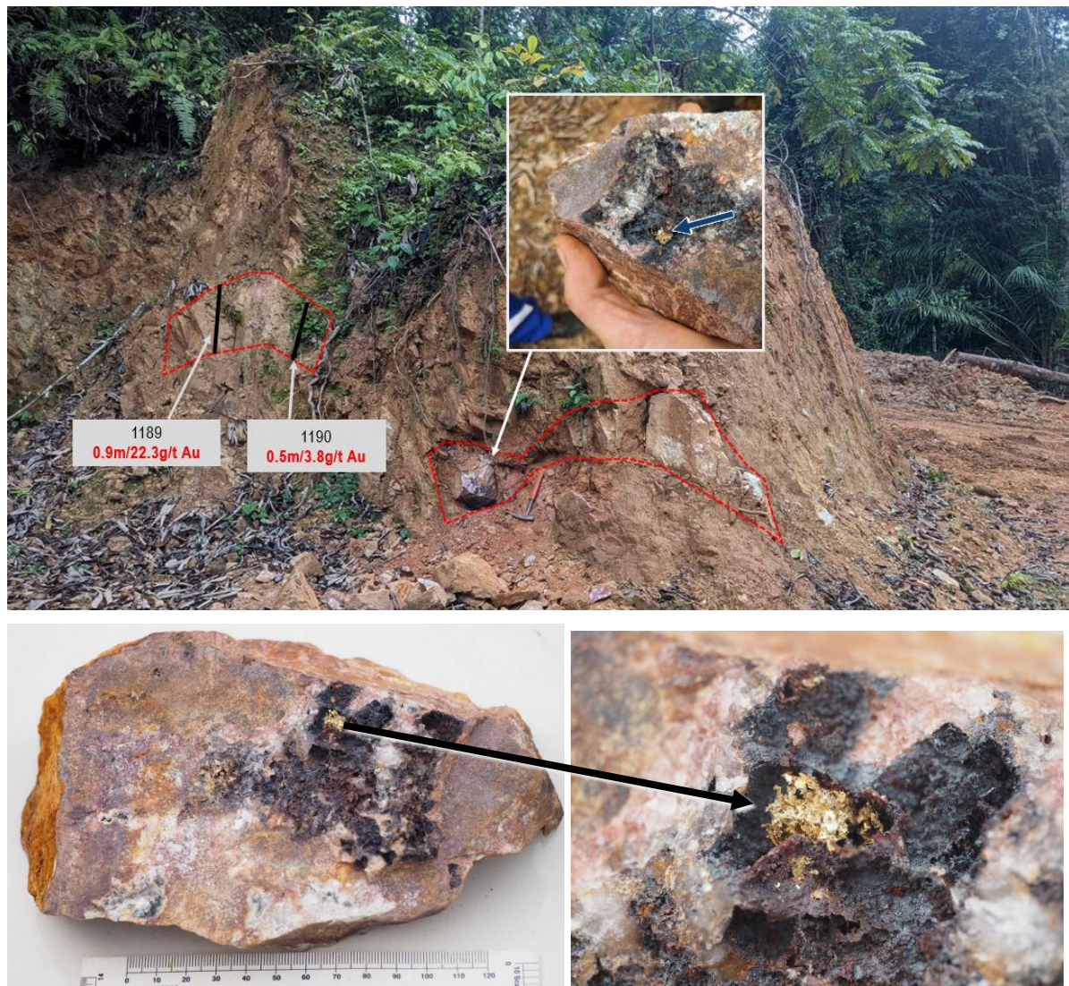
Figure 2: Mineralised quartz vein recently uncovered at A1 drill pad 1
