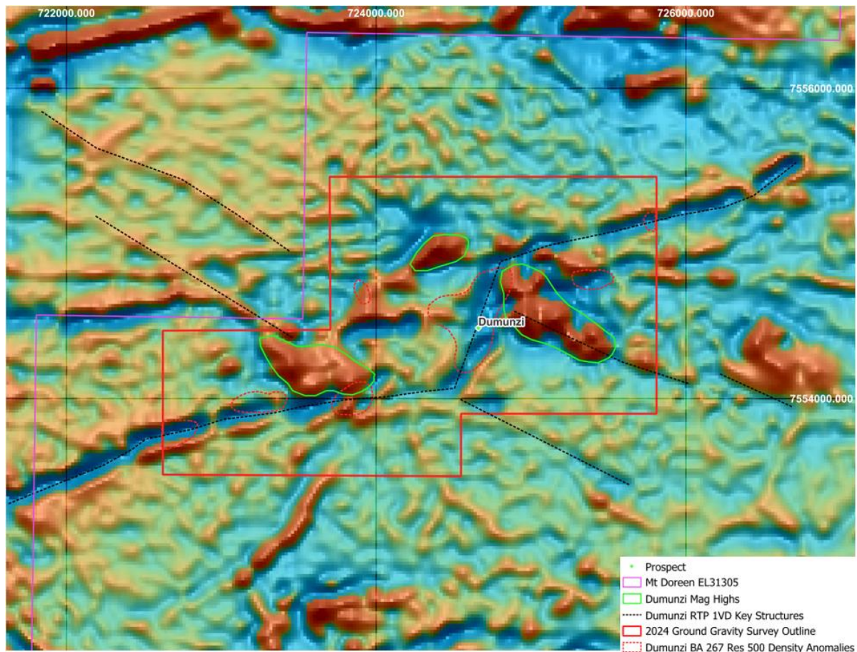
Figure 4 – Showing the large gravity anomaly sitting in the dilation jog at Dumunzi
