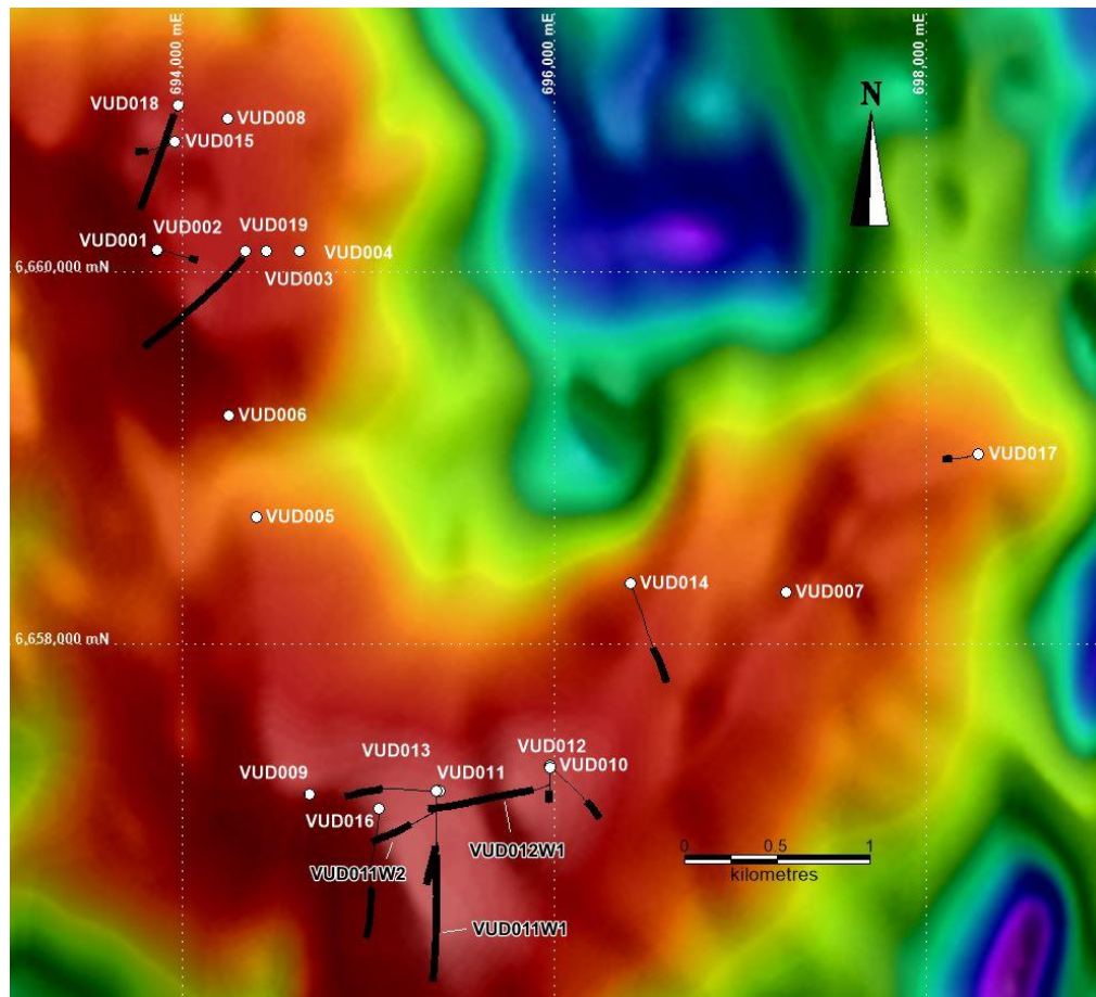
Figure 13: Vulcan Prospect, Fortescue residual gravity image showing location of Vulcan South target area, Fortescue holes VUD0018 & VUD0019 and more recent Vulcan South wedge holes VUD0011W1, VUD0011W2, VUD012W1 and previous Tasman drill holes. The thick black lines on the drill hole traces are the surface projections of basement intercepts (Grid GDA 94, Z53).
