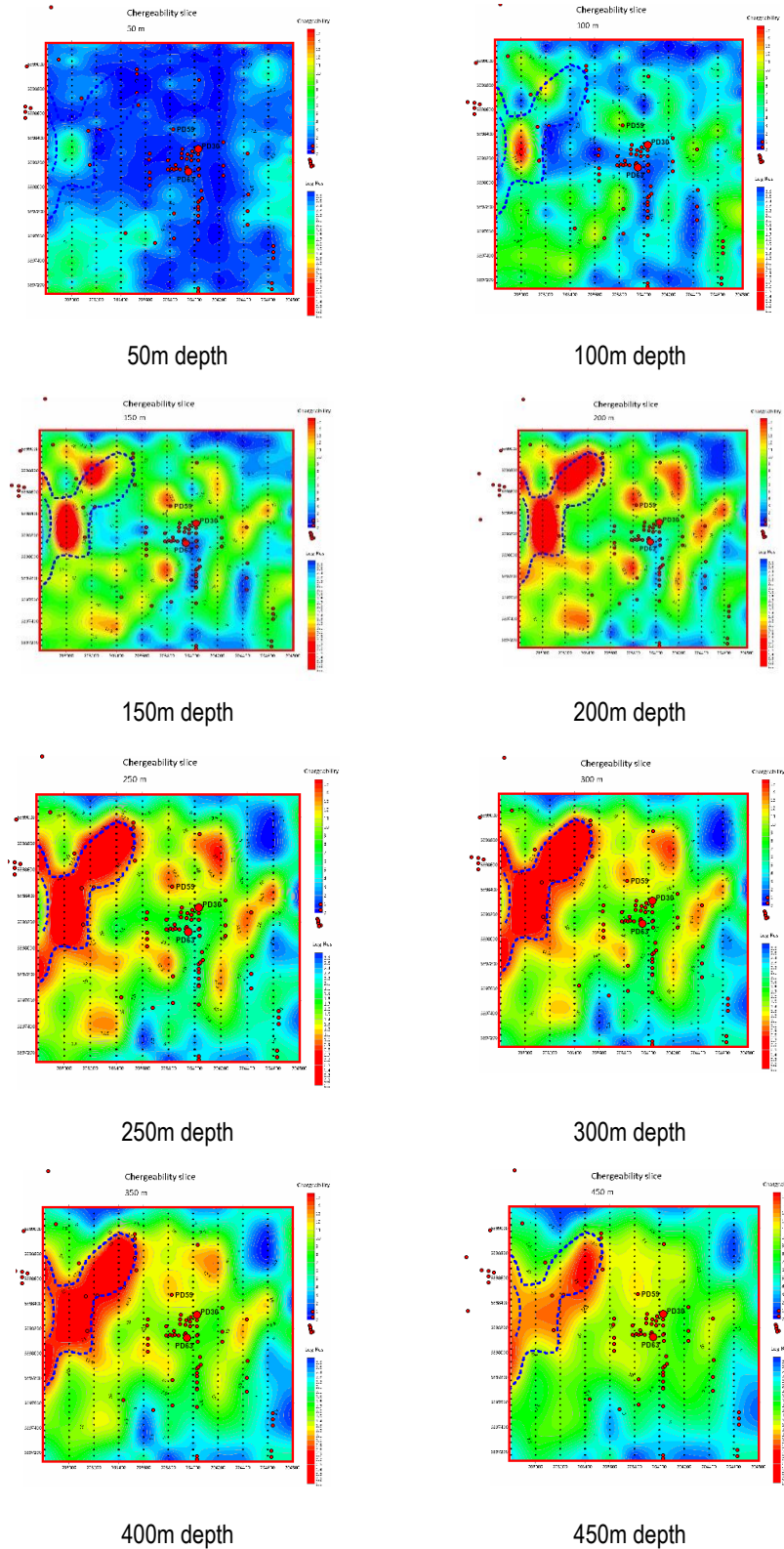
Figure 5a: Montage showing IP Chargeability slices from 50 to 450m. Red boundary is limit of IP survey shown in Figure 3. Blue dashed line is outline of IP anomaly at 300m depth. Previous drill holes are small red dots (refer Figure 1).
