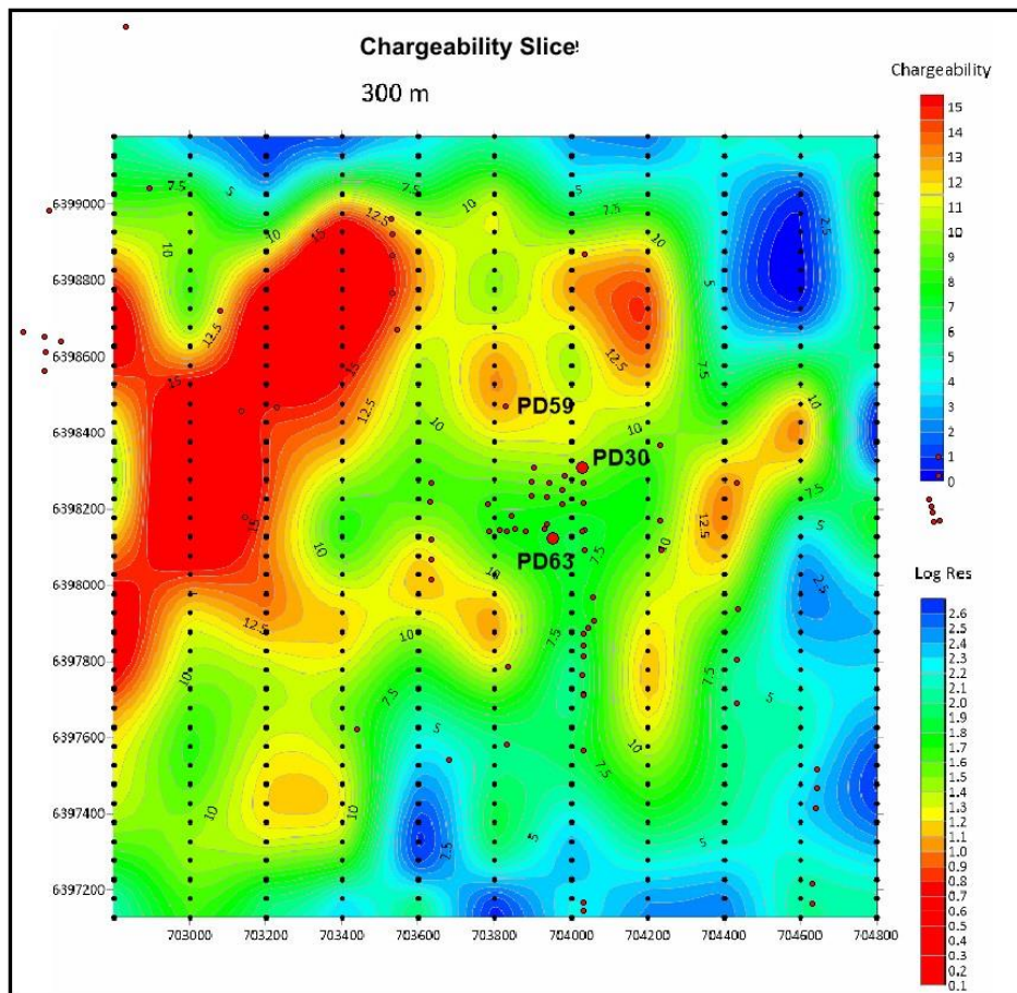
Figure 4: IP Chargeability Slice at 300m depth showing drill hole locations (red dots, not the black dots along the survey lines). Grid MGA2020 Zone 53.
