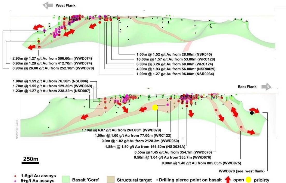
Figure 4 Targets and drilling at Wildwood. Interpreted controlling structures are brown. All results are previously released (ASX:NSM 15 Nov 23)
