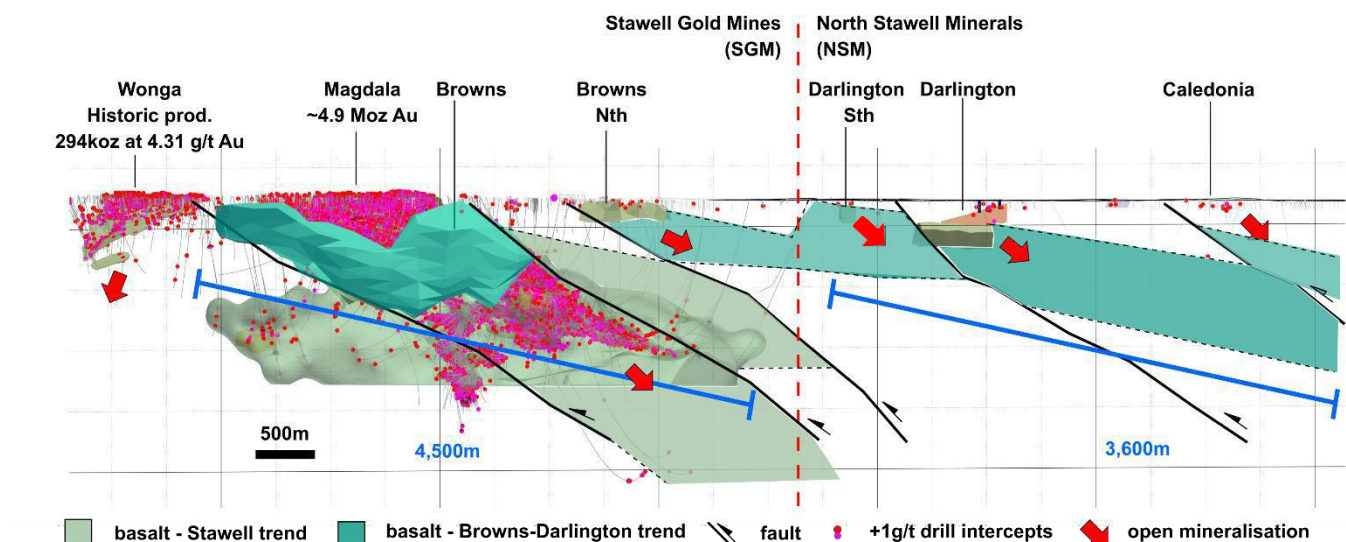
Figure 6 Long-section of the Browns – Caledonia trend. Browns is a basalt dome, sub-parallel to Magdala at Stawell, and the trend may represent a regional gold mineralisation target.
