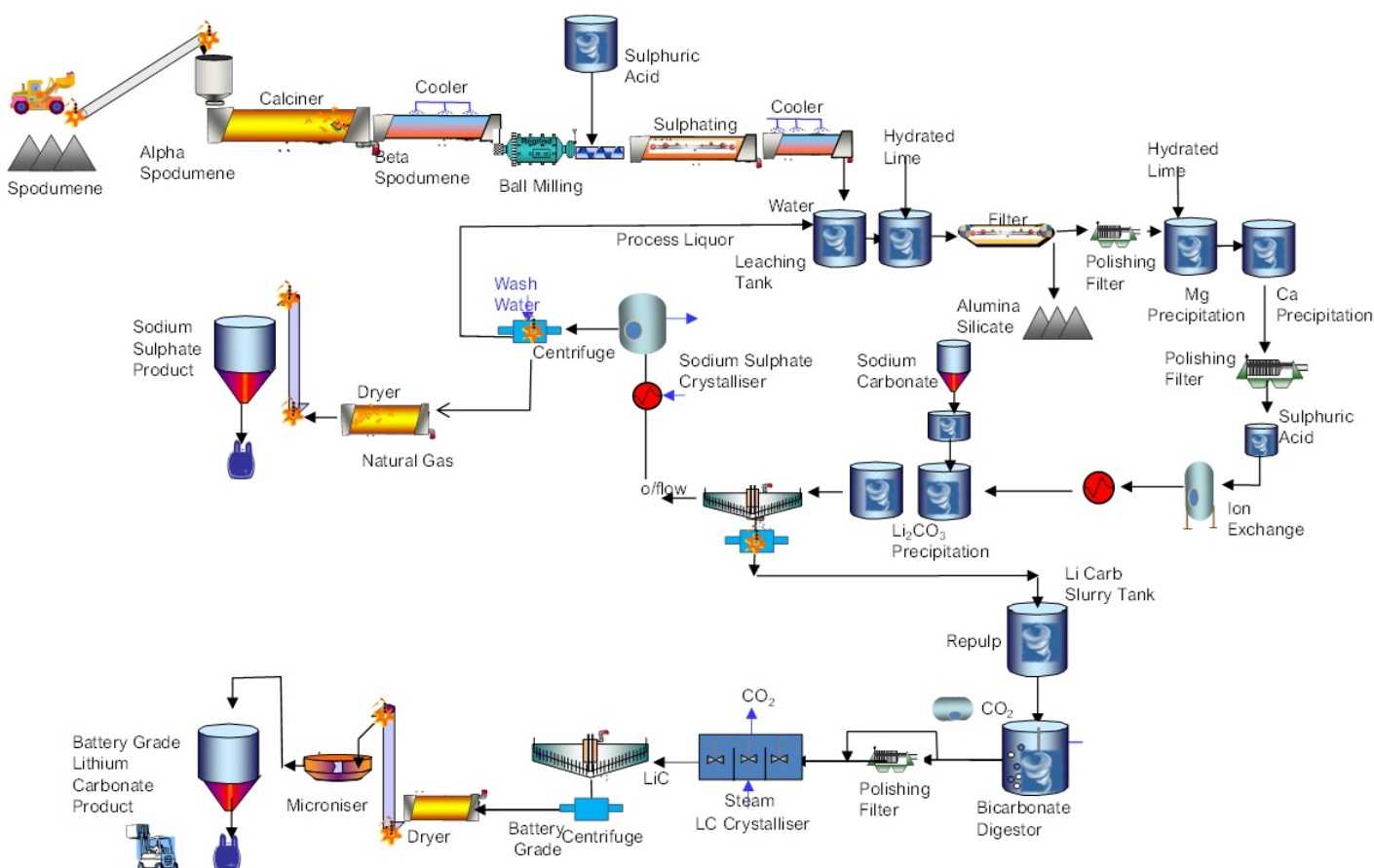
Figure 8: Lithium Universe Bécancour Process Flow Sheet
