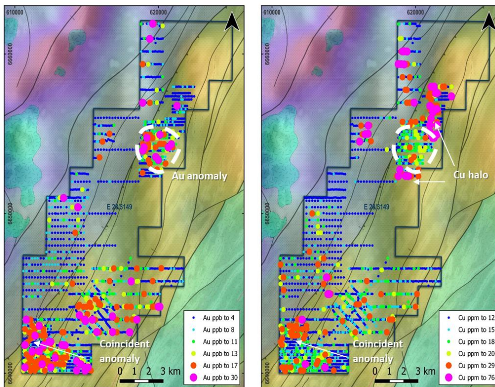
Figure 1: Historical auger assays showing gold and copper anomalies at E28/3149 in the Goldfields.
