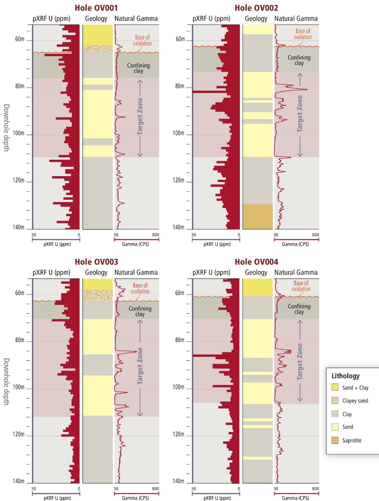
Figure 4: Anomalous downhole pXRF and natural gamma logs over target intervals.
