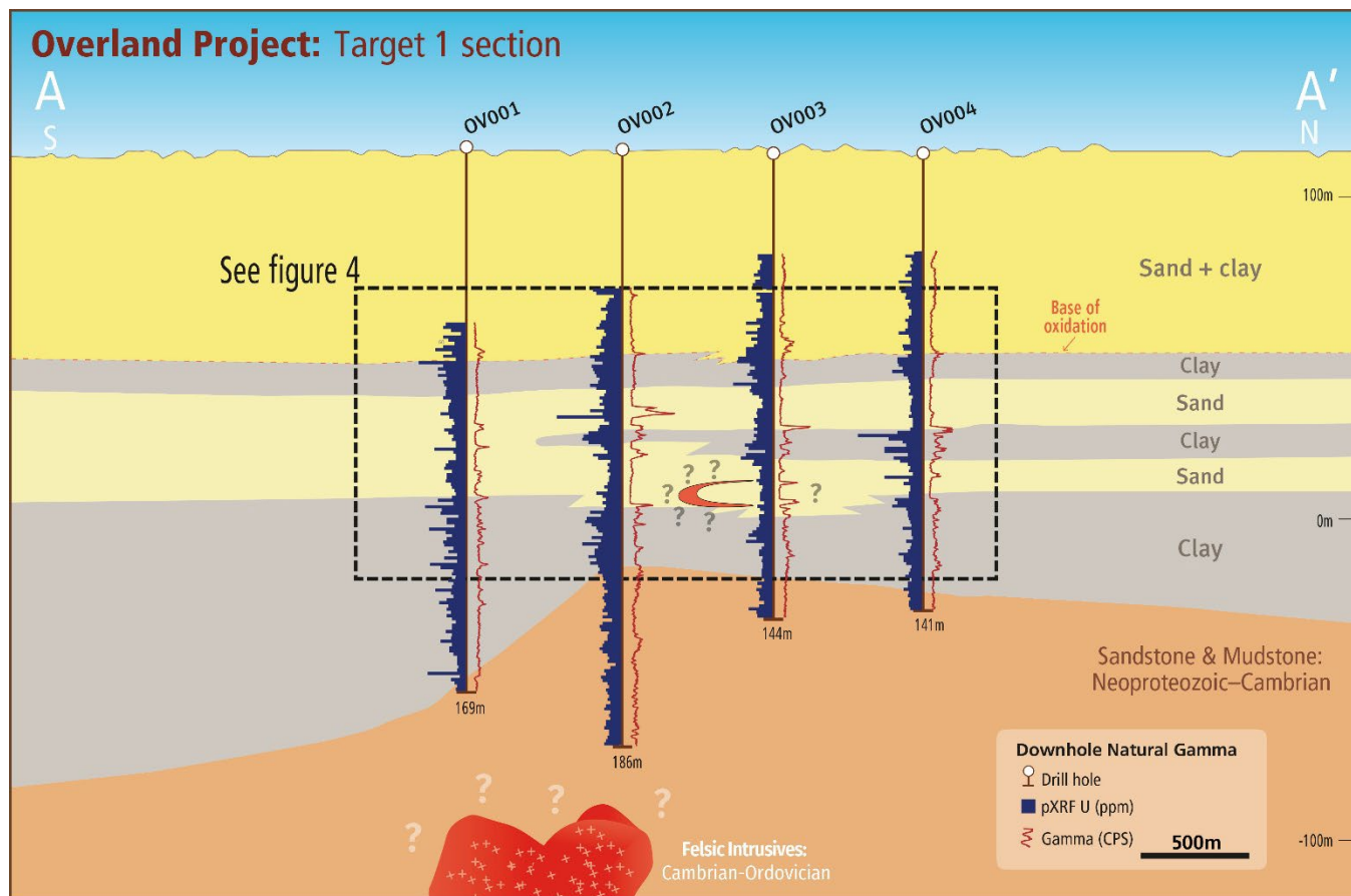
Figure 3: Cross section A-A' showing OV001-OV004 lithology, pXRF U (ppm), Gamma (cps) and Interpreted roll front.
