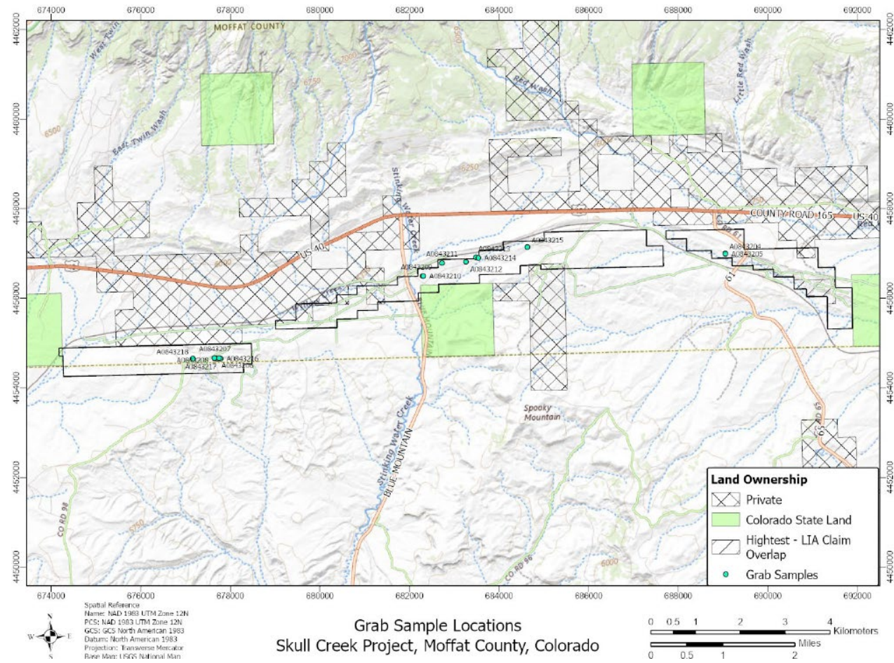
Figure 6: Location of rock chip samples taken from Skull Creek Project
