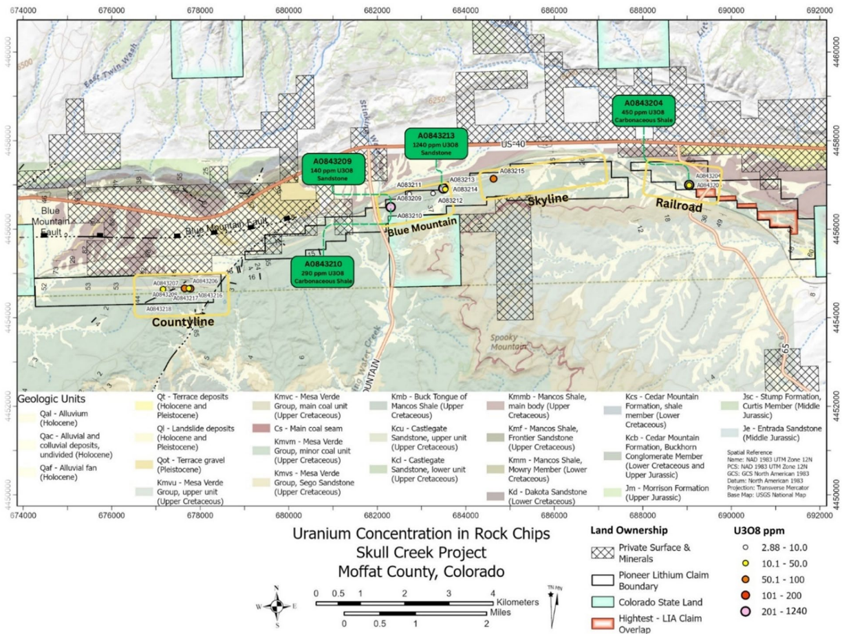
Figure 4: Map showing rock chip samples taken during initial first pass surface exploration of the Skull Creek Project that returned an assay result of greater than 100 ppm U 3 O 8 .
