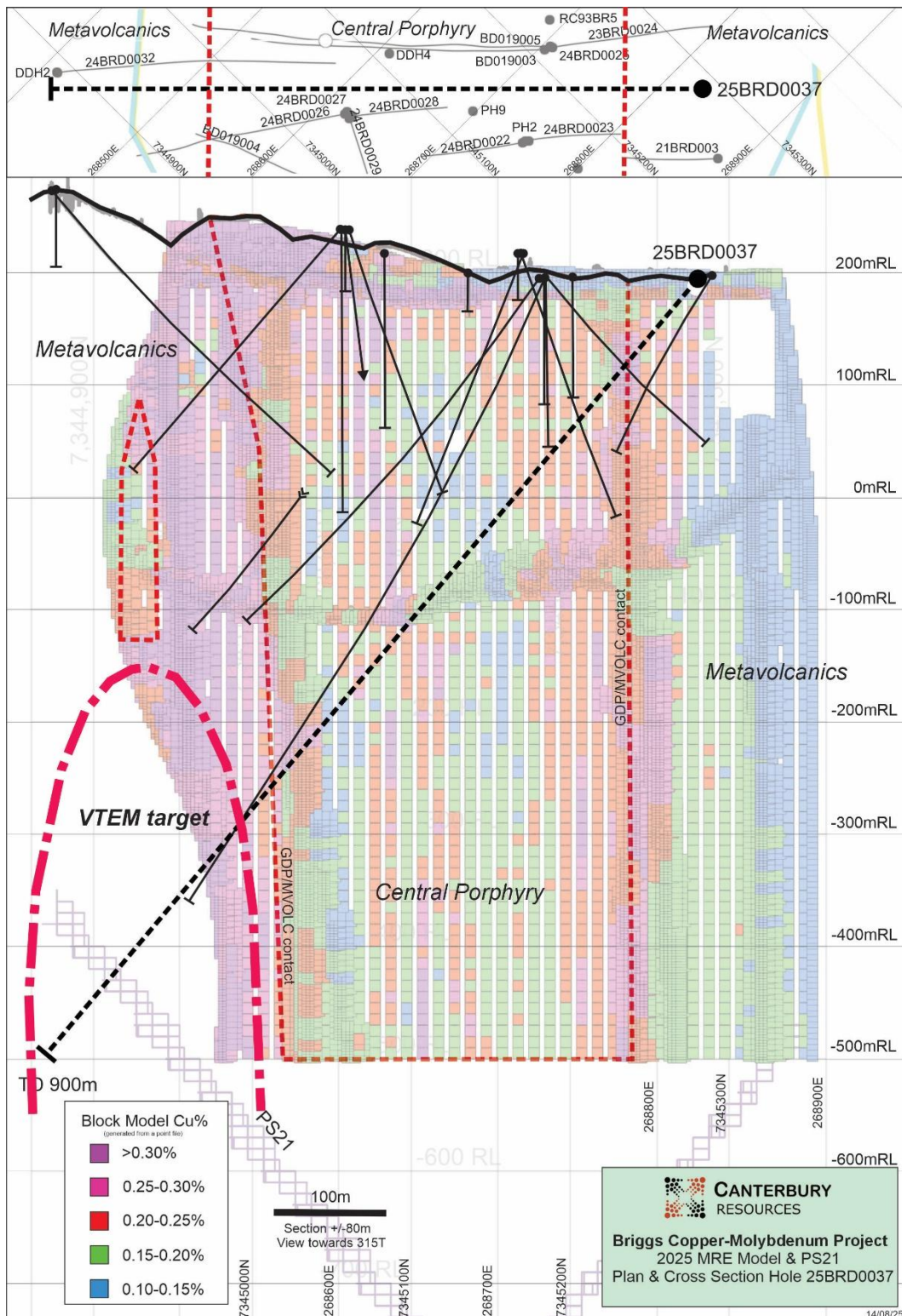
Figure 6 Cross-Section view along the planned trace of hole 25BRD0037 showing block model grade distribution from the 2025 MRE and the outline of the VTEM target.
