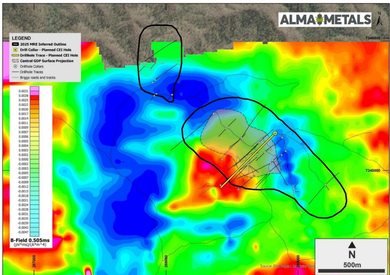
Figure 5 Plan view of the Briggs deposit showing the outline of the MRE, drill collars and the planned deep CEI hole trace on a background image of the B-field of the VTEM electromagnetic survey.
