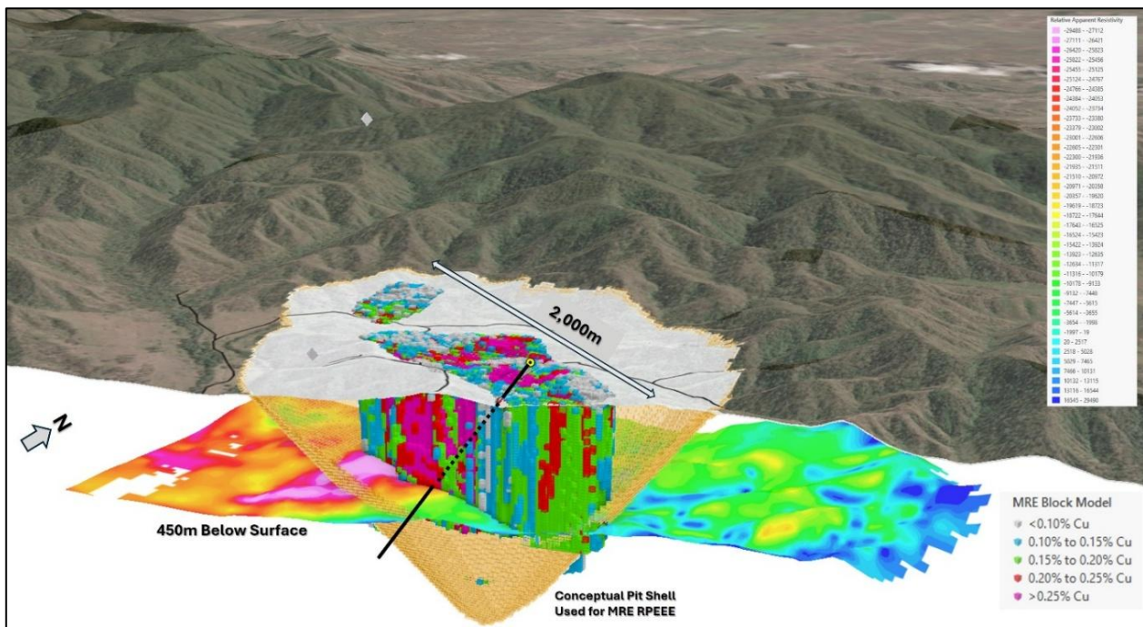
Figure 4 Oblique 3D view showing Apparent Resistivity from the VTEM data at 450m below surface and the juxtaposition of this anomaly with higher interpolated copper grades in the MRE block model.
