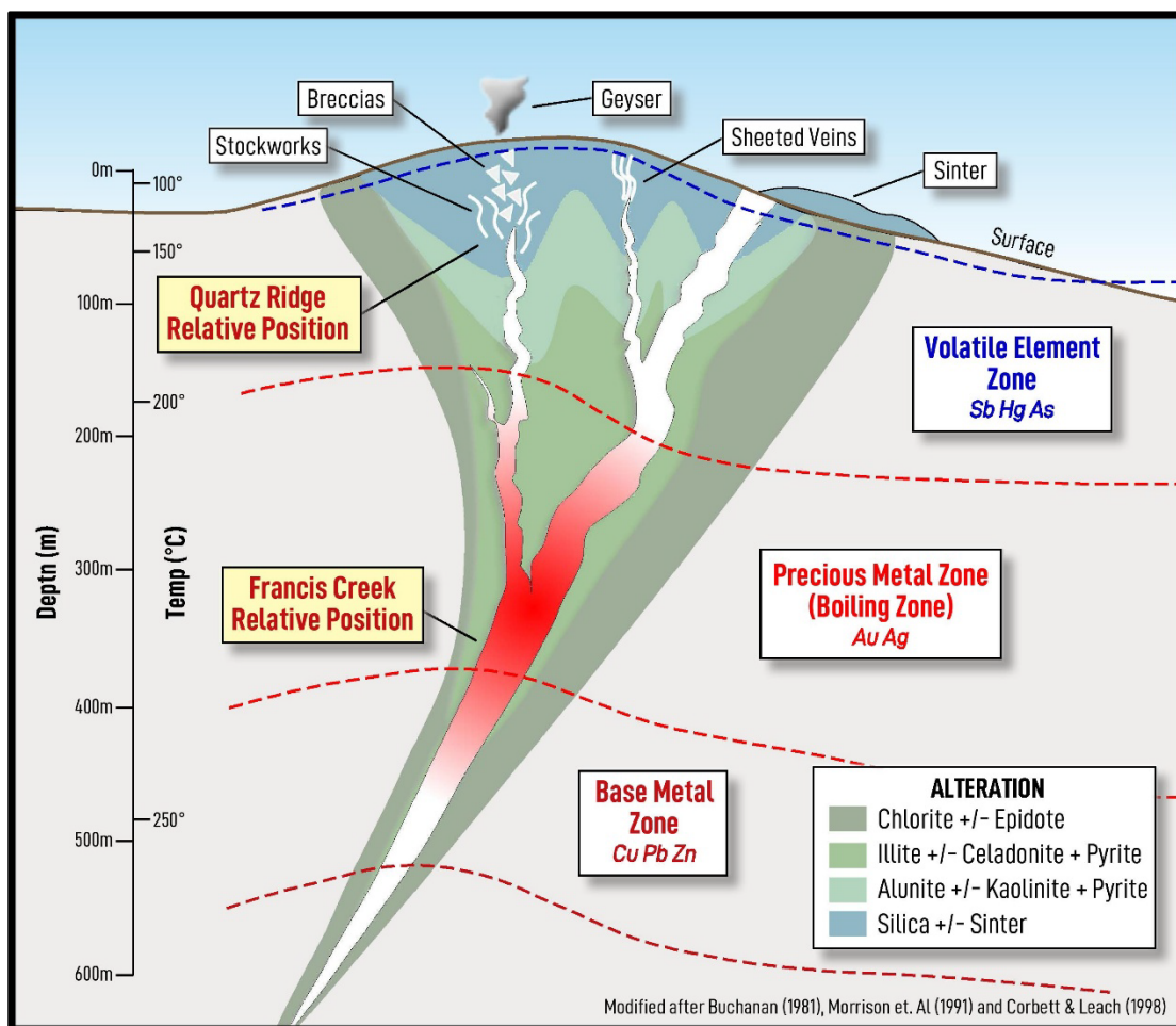
Figure 7: Geochemical zonation in low-sulphidation, epithermal deposits.
