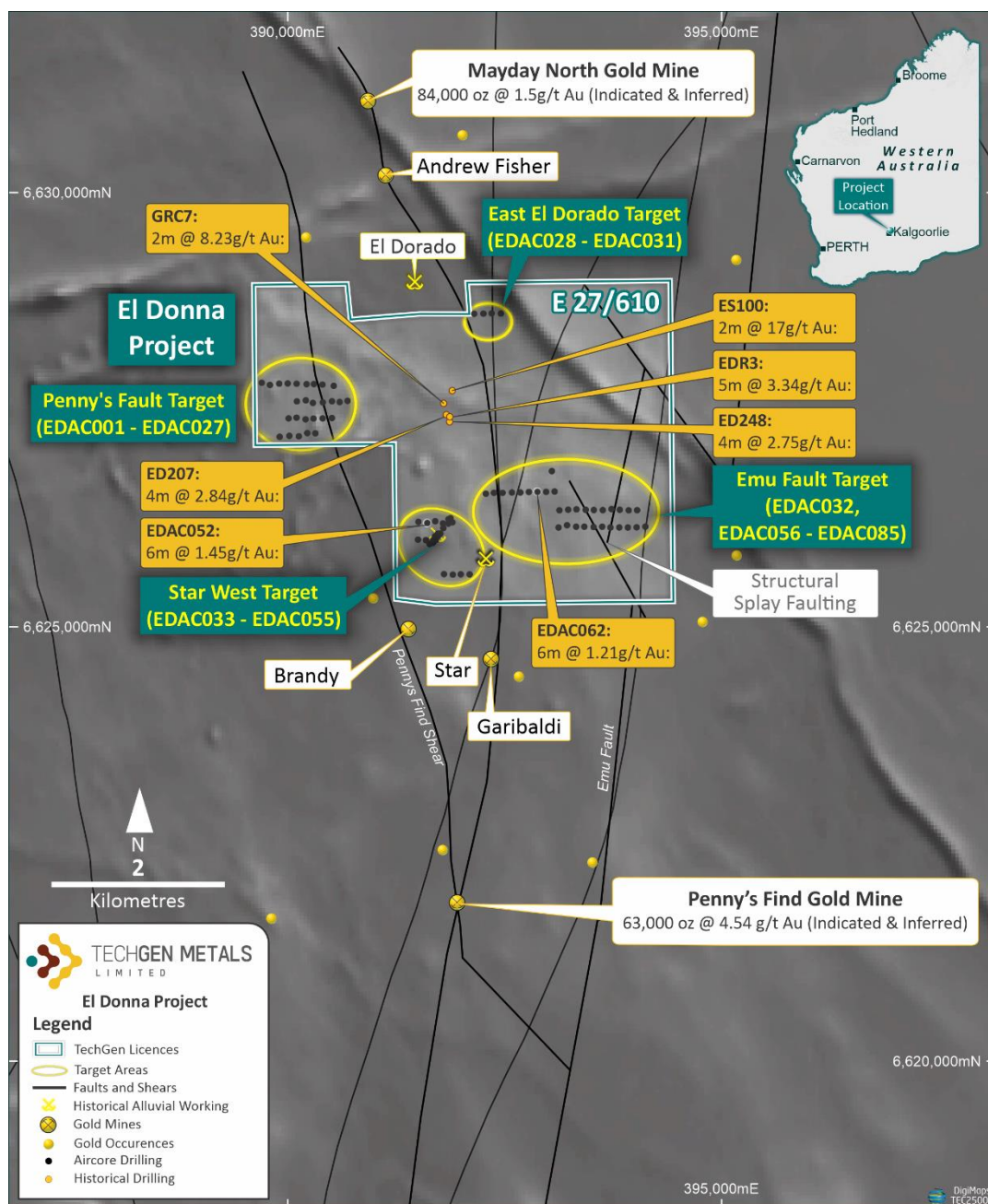
Figure 10: Location of the El Donna Project in between the Mayday North and Penny's Find open pit mines.
