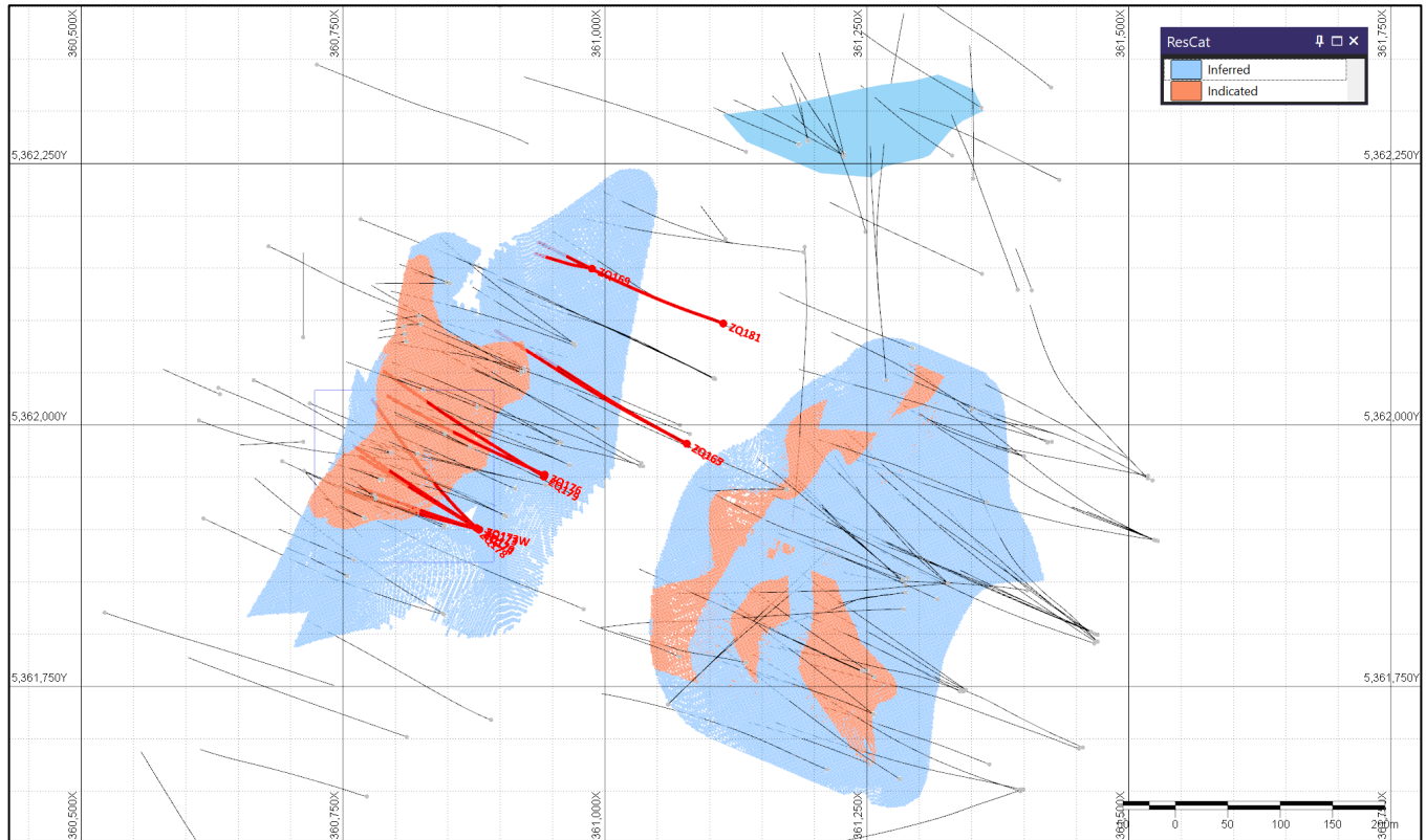
Figure 2: Drill holes from which samples were selected down hole for ore sorting test work.
