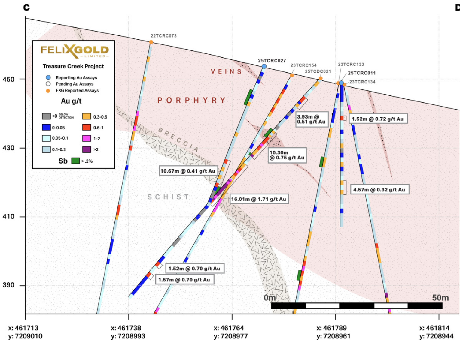
Fig. 4 Section C – D showing gold intersections reported in this announcement and gold assay results from previously reported holes drilled during campaigns in 2022 and 2023.
