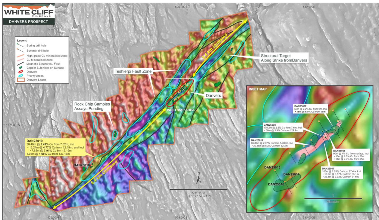
Figure 3 - Map of preliminary magnetic data for the Danvers Project, collect during the 2025 Heli-TEM survey. Newly identified targets are highlighted along strike of Danvers and in similar structural/magnetically quiet zones within the regional Teshierpi Fault Zone, which trends NE/SW over 10km through the Project. (Magnetic basemap is reduced to pole, total magnetic intensity with a NE sun shade overlying DEM. NAD83/UTM Zone 11N).
