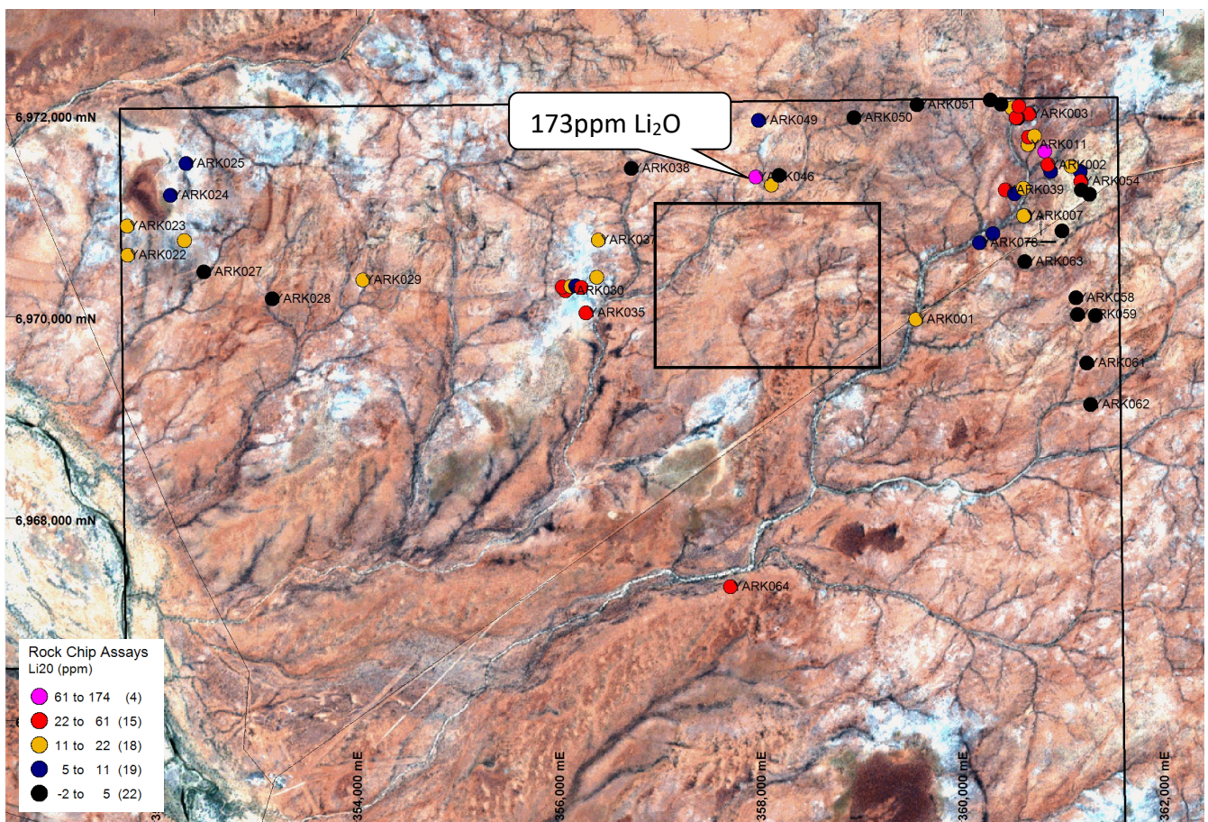
Figure 11. Northern end of North block of E70/5464 showing sample locations and \text{Li}_2\text{O} results in relation to tenement outline and box indicating where follow up sampling is required.
