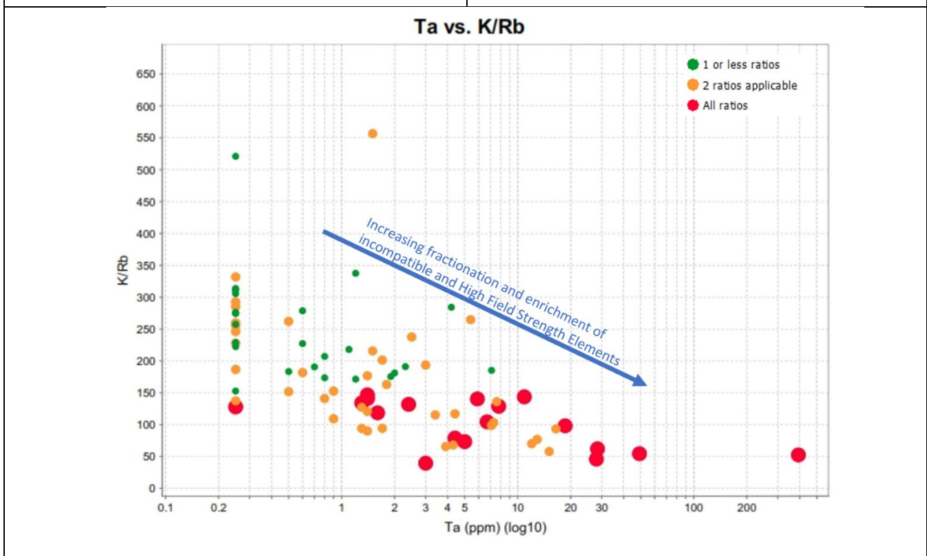
Figure 9: Ta (ppm) versus K/Rb plot from Llama property, highlighting the relative degree of fractionation in the collected samples ( 5 Steiner et al. 2018). Symbology as per 4 Ballouard et al. (2016) where red indicates samples with elemental ratios of K/Rb<150, Nb/Ta<5 and Zr/Hr<18, orange indicates 2 out of 3 ratios are true and green indicates 1 or less ratios are applicable. Ta (ppm) axis log 10 for scale.
