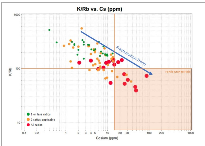
Figure 7: K/Rb versus Cs - for Llama pegmatite samples showing clear fractionation towards and into fertile granite field. Symbology as per 4 Ballouard et al. (2016) where red indicates samples with elemental ratios of K/Rb<150, Nb/Ta<5 and Zr/Hr<18, orange indicates 2 out of 3 ratios are true and green indicates 1 or less ratios are applicable.
