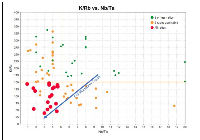
Figure 8: K/Rb versus Nb/Ta fractionation ratios with Llama assay results. Orange lines indicate zone where K/Rb<150 and Nb/Ta<5 ( 4 Ballouard et al. 2016). Symbology as per 4 Ballouard et al. (2016) where red indicates samples with elemental ratios of K/Rb<150, Nb/Ta<5 and Zr/Hr<18, orange indicates 2 out of 3 ratios are true, and green indicates 1 or less ratios are applicable.
