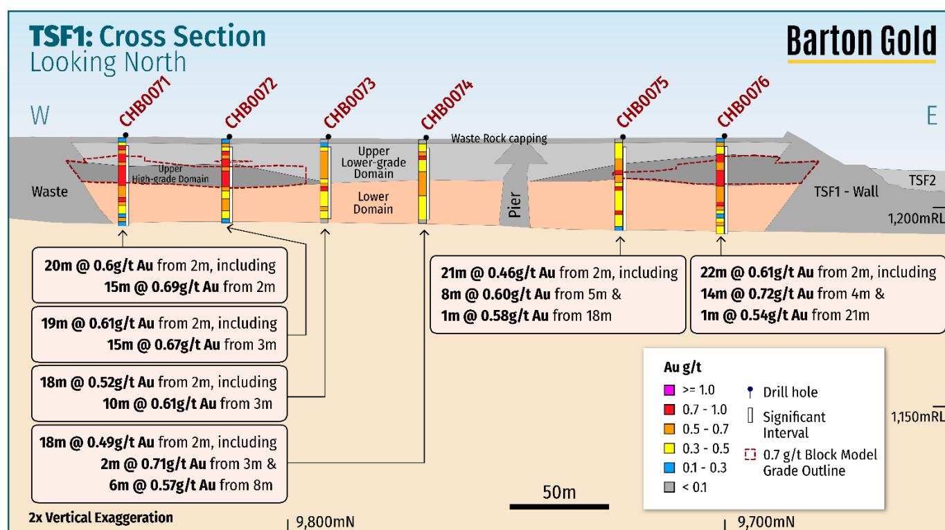
Figure 1 - Cross section showing higher-grade peripheral TSF1 materials & 0.7g/t Au grade shell 1
