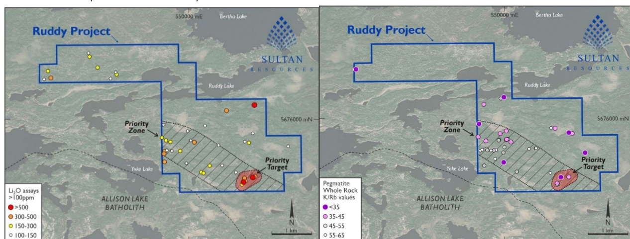
Figure 3 (L) and Figure 4(R): \text{Li}_2\text{O} Assays reporting above 100ppm at Ruddy Project in relation to tenure. Priority Zone area of focus for LCT Pegmatites in hatched area. Pegmatite locations demonstrating lower K/Rb ratios considered indicative of more evolved pegmatitic occurrences, and a vector for LCT pegmatite mineralisation
