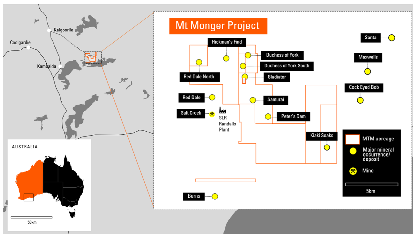
Figure 9: Location diagram of the Mt Monger Project showing tenements and known gold occurrences.
