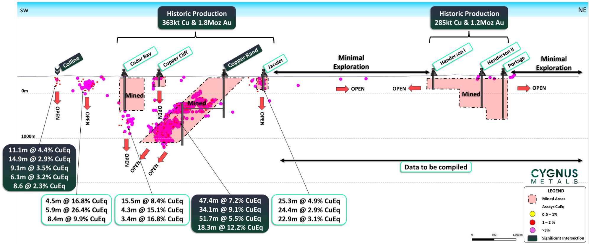
Figure 3: Long Section through the Chibougamau North Camp illustrating significant intersections from Colline and Copper Rand in particular, including the standout mined intersection of 47.4m @ 7.2% CuEq at Copper Rand. 4
