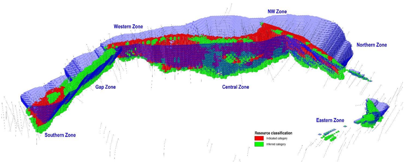
Figure 5 – Perspective view of Kokoseb, looking towards the NW, showing resource categories in the block-Model
