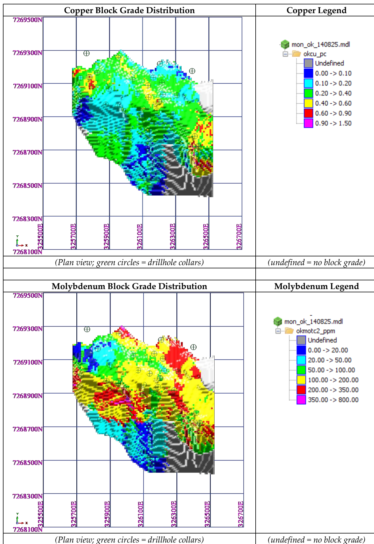
Figure 9 Copper and Molybdenum Block Grade Distribution
