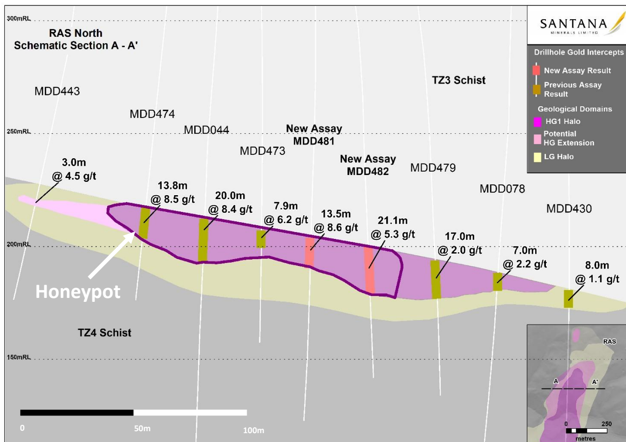
Figure 2. Schematic cross section at 5018150N showing high grade intersections
