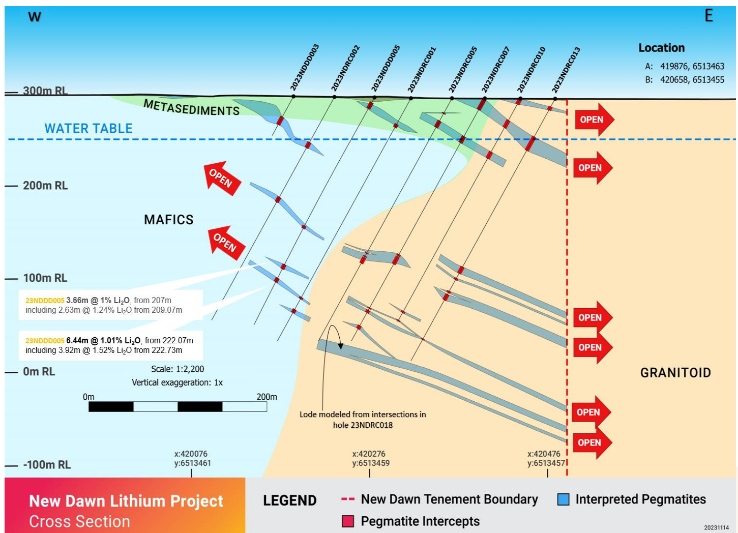
Figure 9 New Dawn Lithium Project. Cross Section showing current drilling and pegmatite intersections
