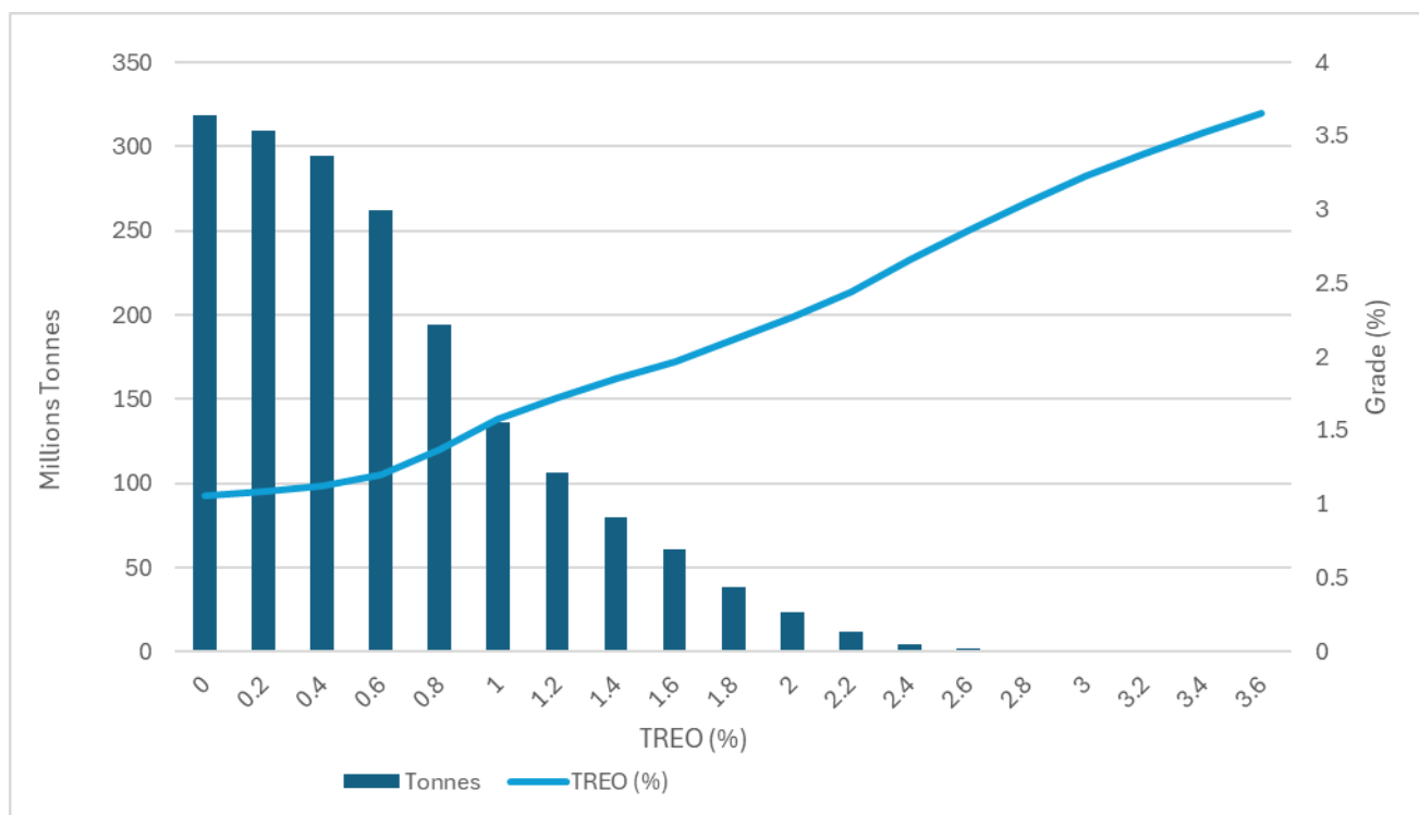
Figure 7 – Grade tonnage curves Inferred
