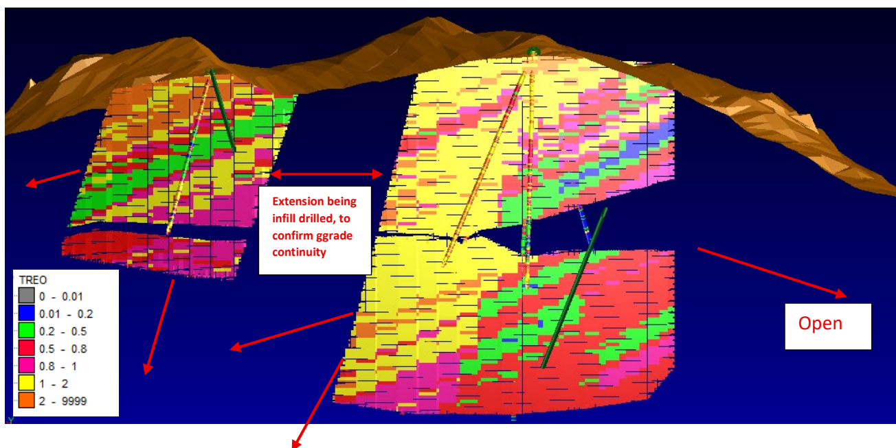
Figure 8 - Block Model images
