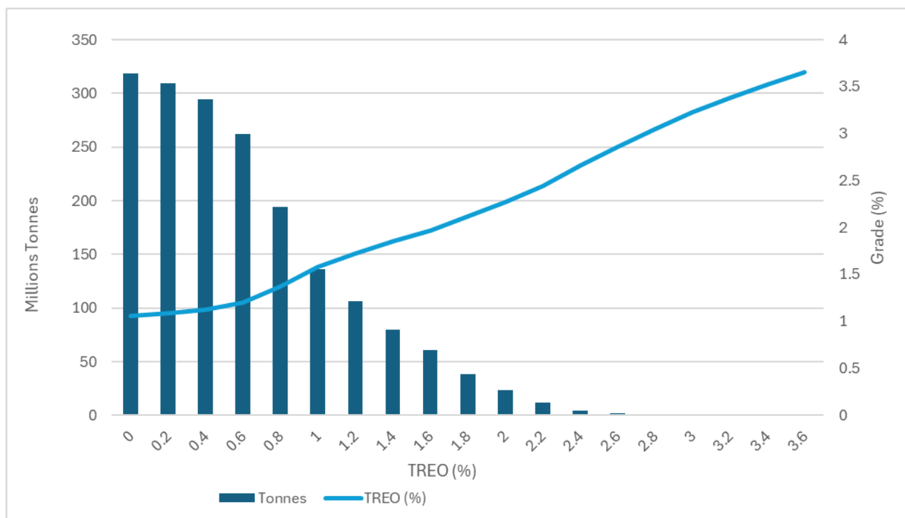
Figure 8 – Grade tonnage curves Inferred
