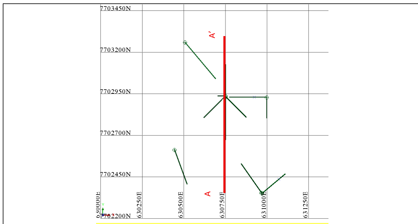
Figure 5: Plan View of Drill Holes
