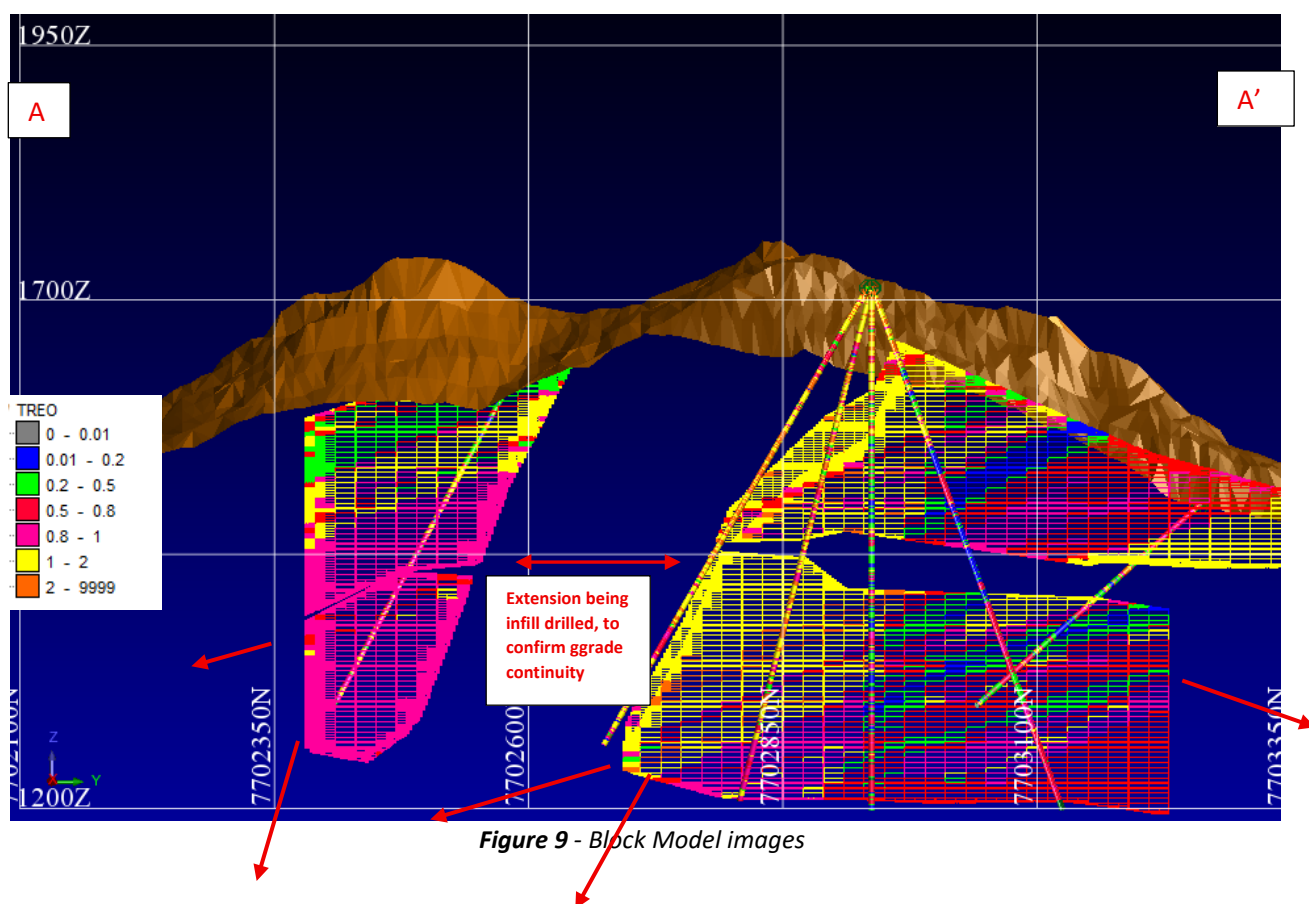
Coloured holes included in MRE, Green awaiting assays Sectional View of MRE Showing Open in all Directions
