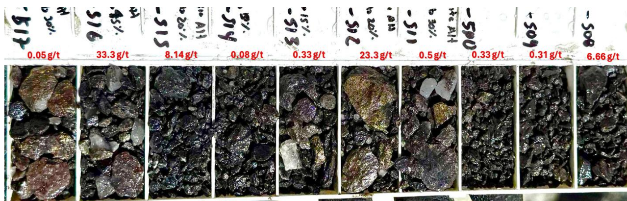
Figure 3 RC chips, hole 25PRC178: abundant pyrrhotite, chlorite alteration and quartz-carbonate veins; 5m @ 13 g/t Au from 512m. The hole appears to have entered and exited the mineralised zone.
