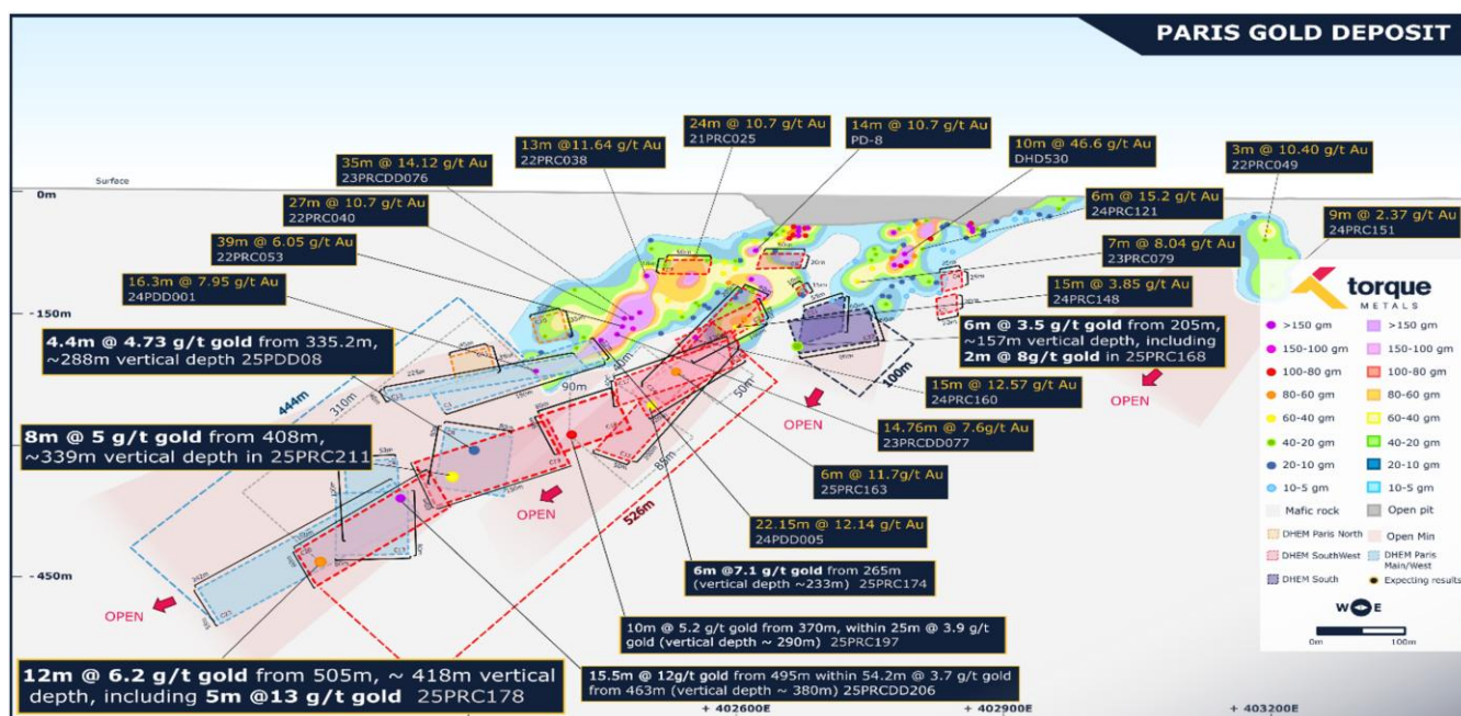
Figure 1 EM conductor plates modelled from DHEM surveys targeting extensions of pyrrhotite-associated gold mineralisation.
