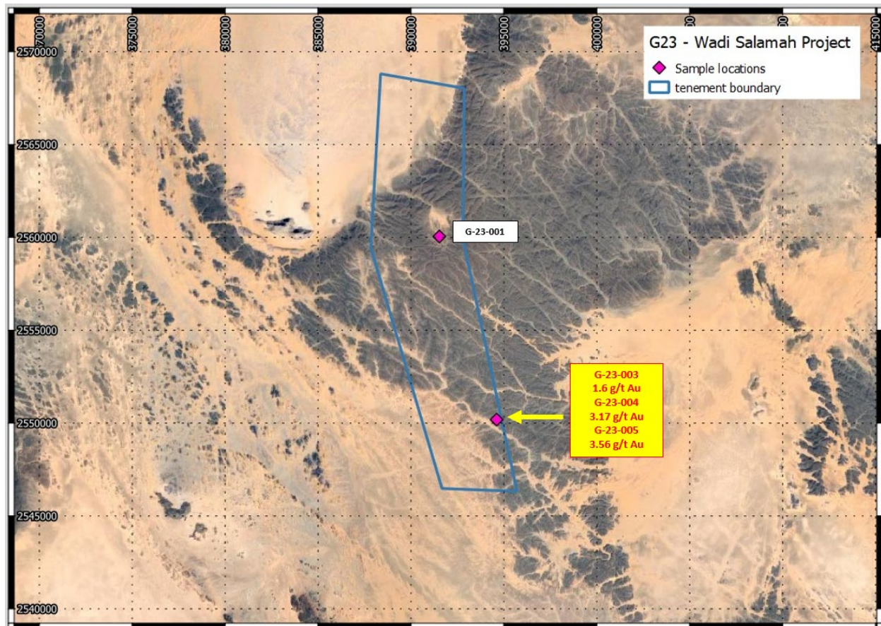
Figure 1: G-23 (Wadi Salamah) sample locations
