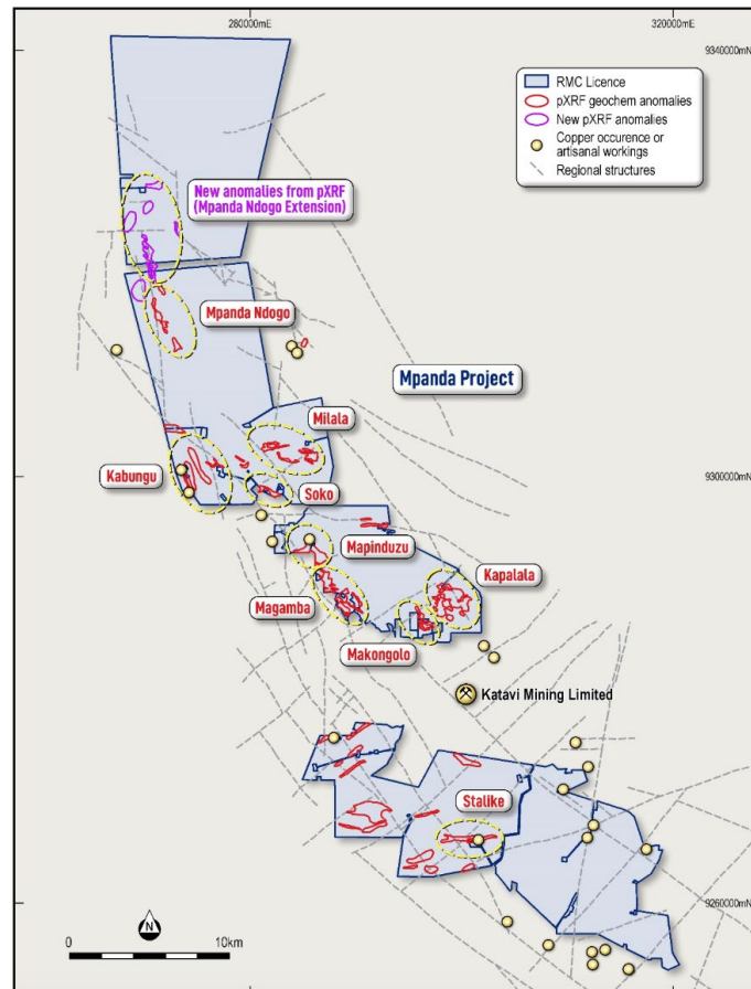
Figure 3: Mpanda Project Anomalies including the Katavi Copper Mine location
