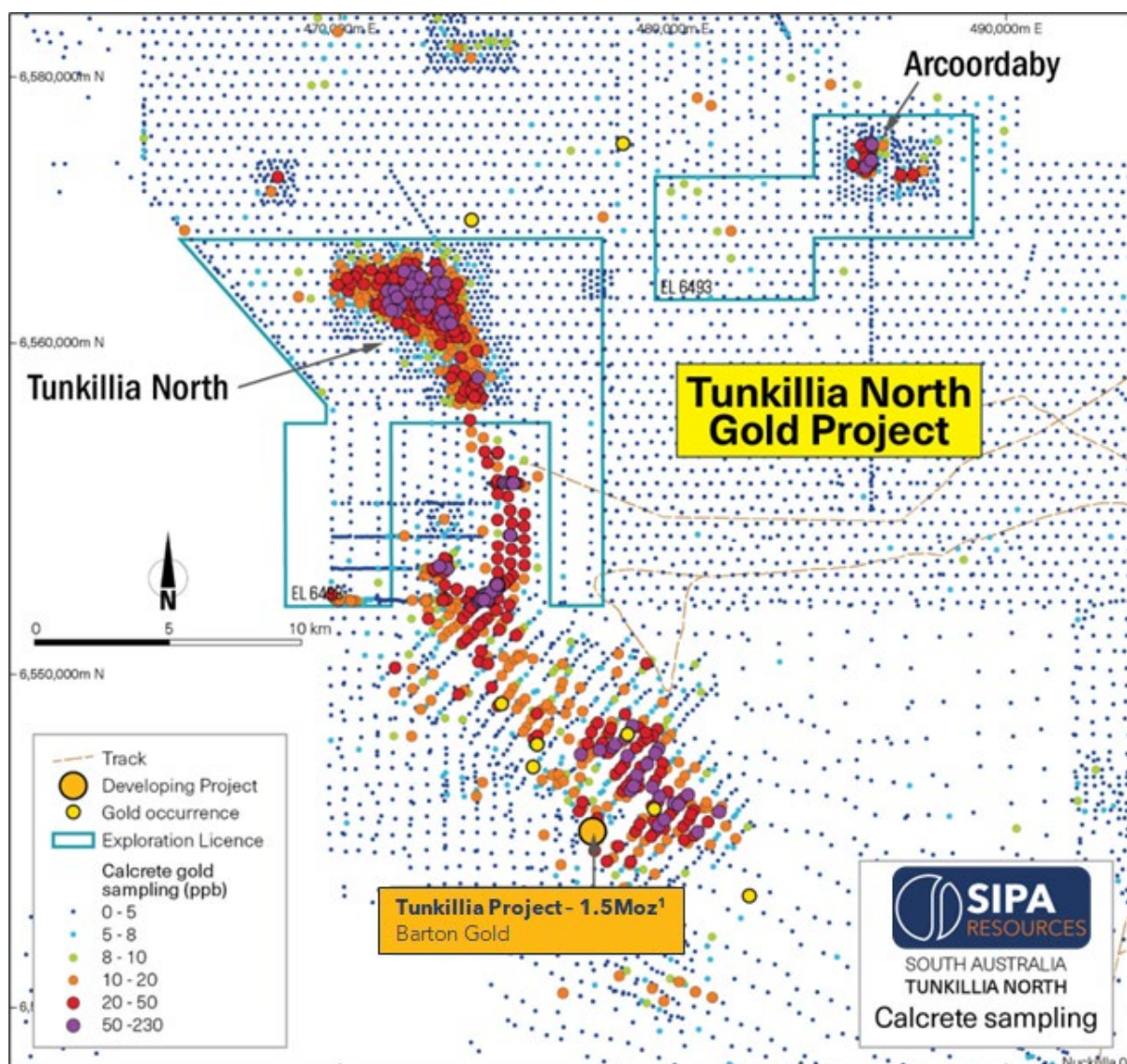
Figure 4: Tunkillia North Historical Gold-in-Calcrete Geochemistry
