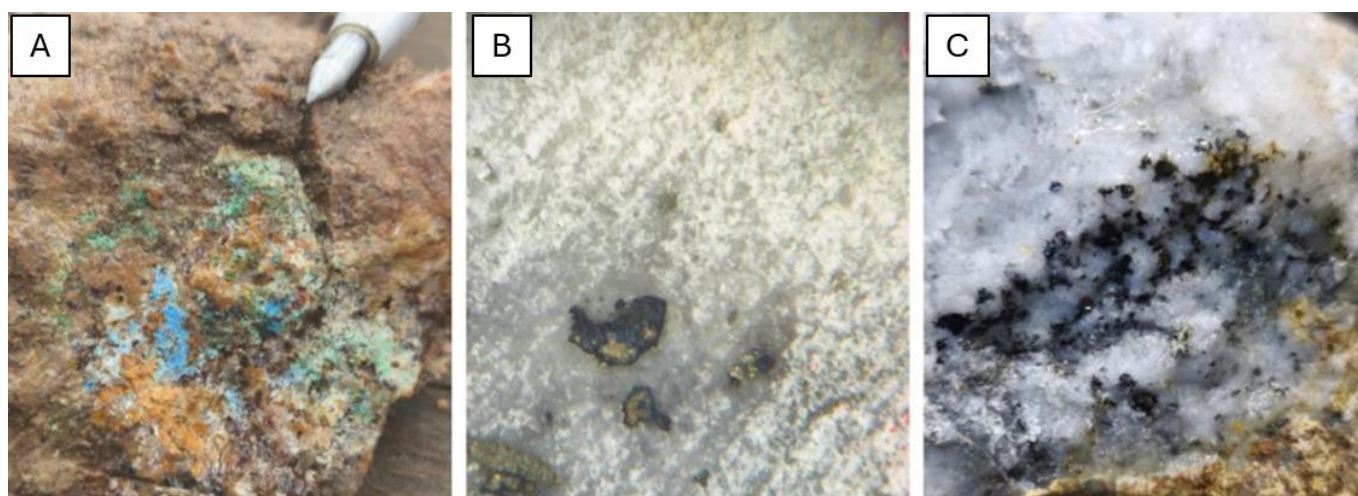
Plate 2. Mineralization examples taken from the epithermal vein system in trench CVT25-022. A.) Supergene enrichment zone malachite and azurite. B.) Microscopic view of chalcocite replacing chalcopyrite. C.) chalcocite with sulphides.
