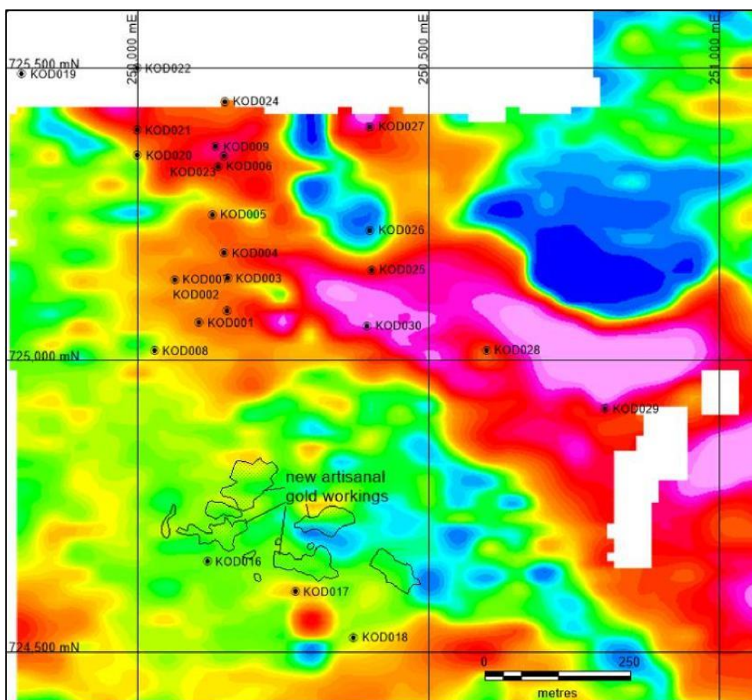
Figure 2 – Drill locality plan on map of gradient array IP (red/magenta colors indicate anomalies). Note: holes KOD001-009 were drilled in the 2016 drill program.
