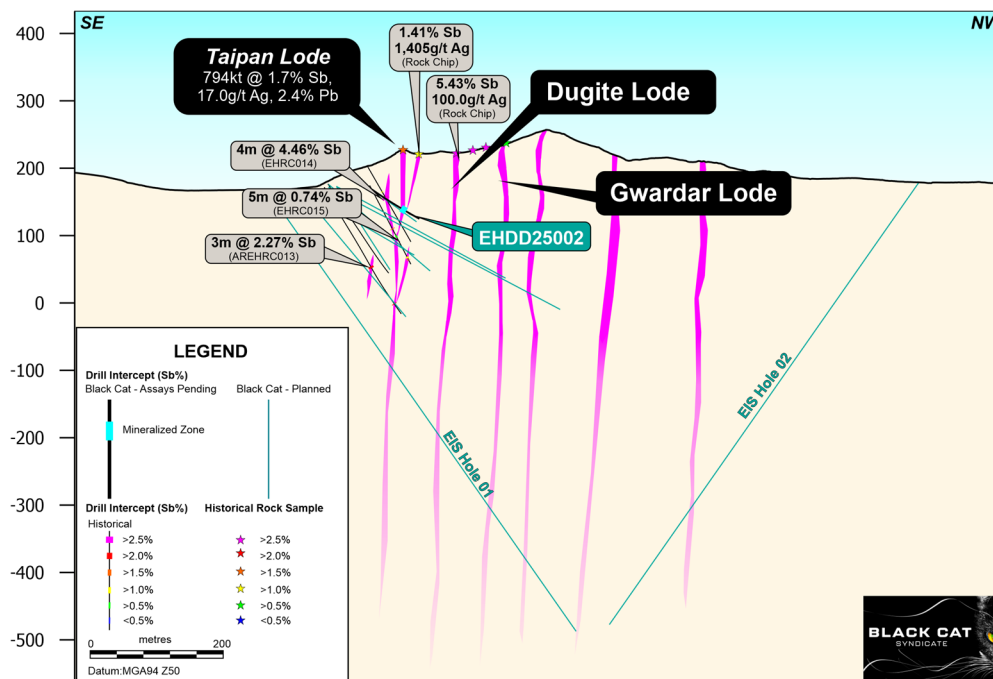
Figure 2: Cross section through Mt Clement showing historical drill results and surface samples, interpreted lode extensions and planned EIS-co-funded drill holes.
