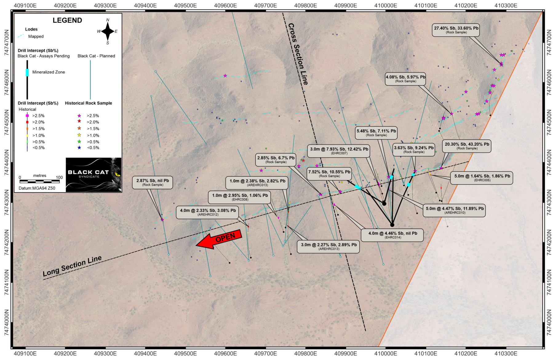
Figure 3: Plan view showing historical drill intercepts and rock chip sample locations 6 at the Mt Clement Antimony Project as well as the locations of current and planned drilling. The mineralized zones intersected in the three current drill holes are indicated and assays are pending for all intervals. The section lines for Figures 2 and 4 are indicated.
