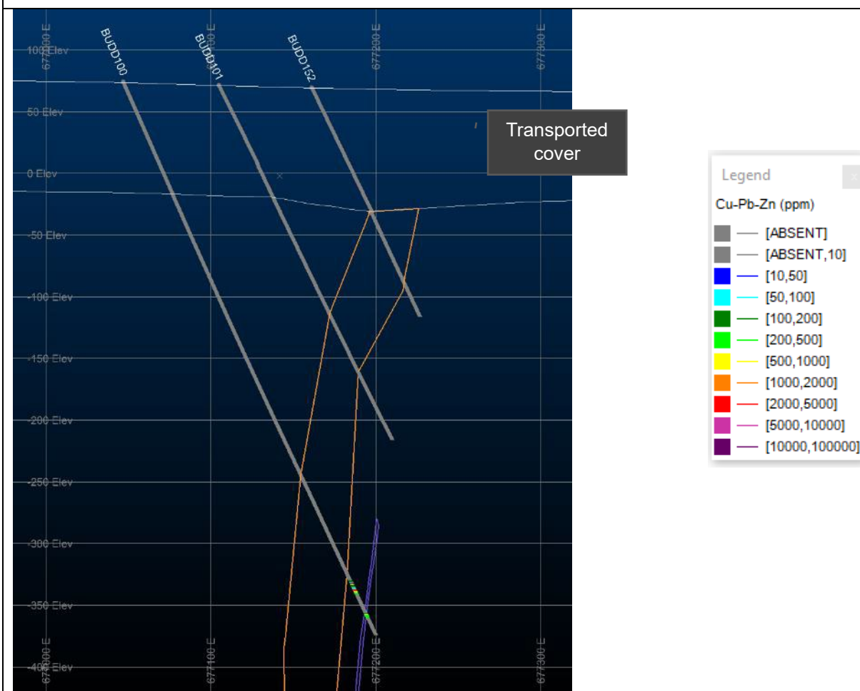
Figure T2. Cross section view showing drill holes and major geological units and assays from this release. Note for details of holes not listed in this JORC Table 1 refer to JORC Table 1 of LML ASX announcement dated 8 July 2025, titled "Minbrie Copper Base Metals Priority Drill Targets Confirmed"
