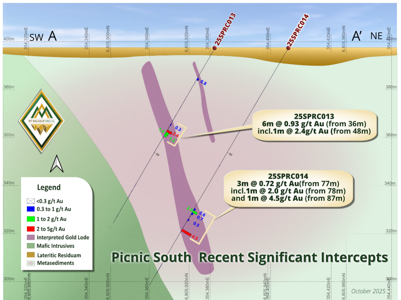
Figure 2: Cross-sections through key recent drill holes illustrating shallow gold mineralisation (Window 50m).
