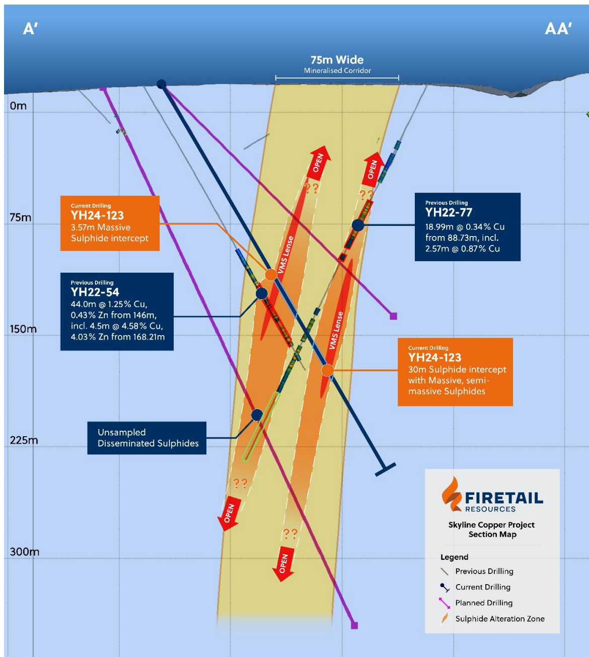
Figure 4: Schematic Cross section of YH24-123 and planned drill holes with historic drill holes
