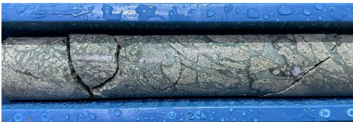
Figure 5: EXAMPLE OF HYDROTHERMAL BRECCIA WITH CHALCOPRYITE, CHALCOCITE AND PYRITE IN DRILL HOLE
