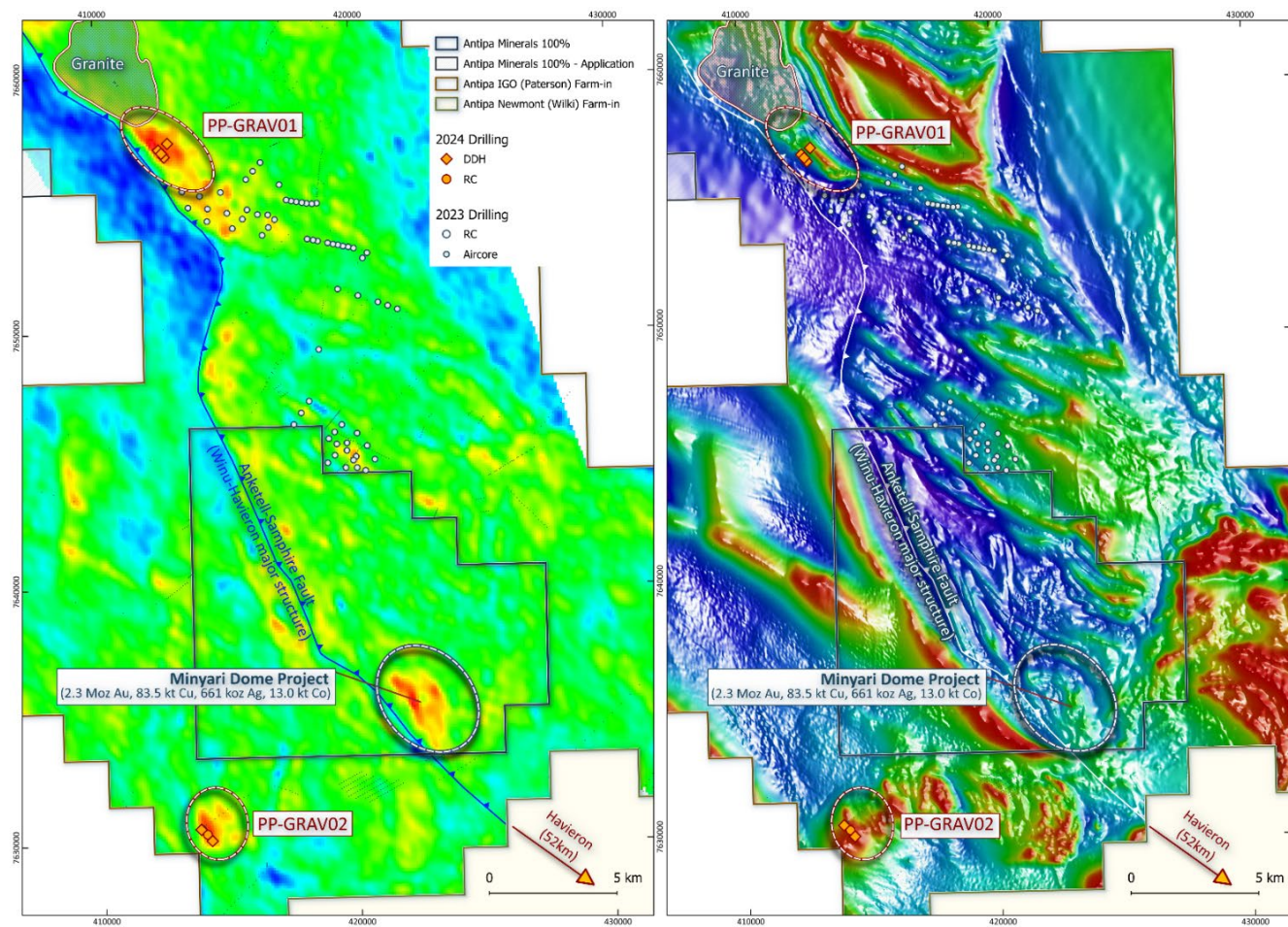
Figure 4: Plan showing the southern region of the Paterson Farm-in Project 2022 Airborne Gravity Gradiometer (AGG) image (LHS) and aeromagnetic image (RHS), showing the location of two co-incident magnetic and gravity high targets PP-GRAV01 and PP-GRAV02 and drill hole locations. Note the location of the Anketell-Samphire Thrust, a possible hydrothermal fluid conduit linking the Winu, Minyari and Havieron gold-copper-silver deposits (combined resources of 17Moz of Au, 4Mt of Cu and 52Moz of Ag) 10 and reduced granites adjacent to both PP-GRAV01 and PP-GRAV02. NB: Regional GDA2020 / MGA Zone 51 co-ordinates, 10km grid.
