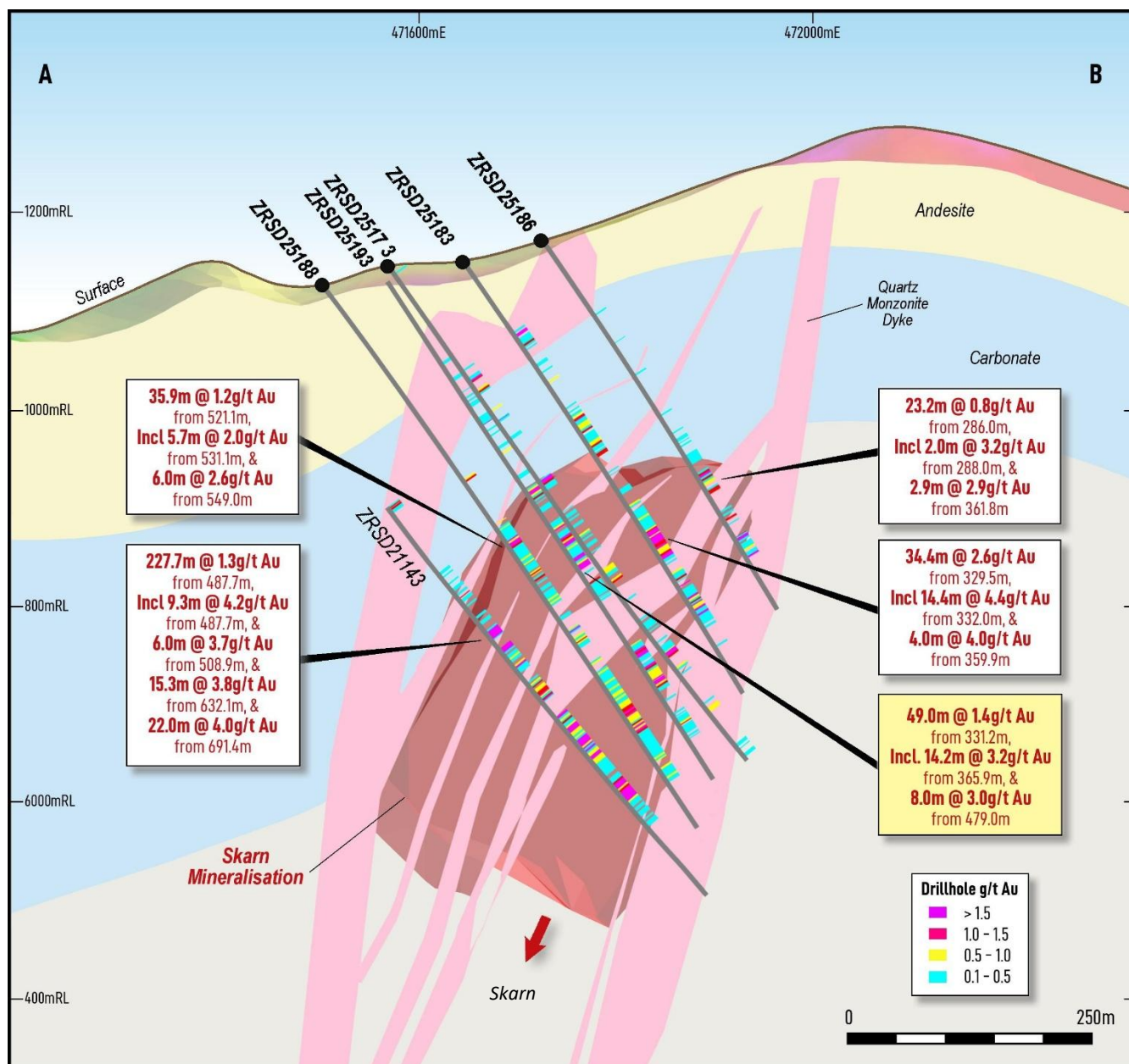
Figure 3. Gradina cross-section view along A-B, showing results for ZRSD25193 in relation to previously reported drill intercepts.
