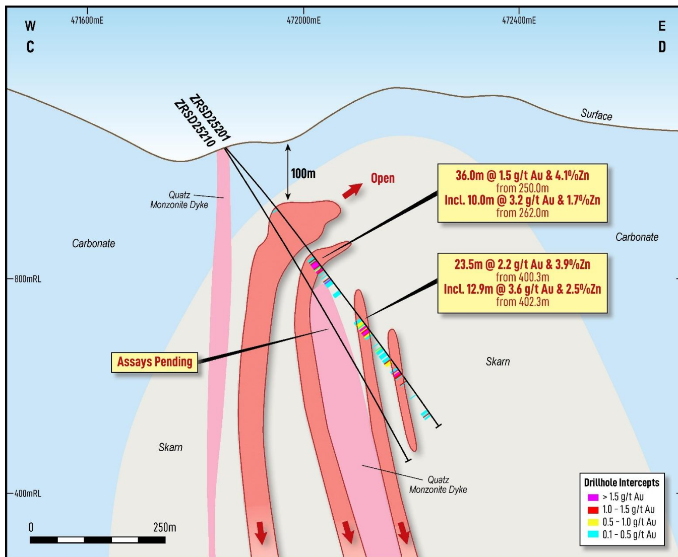
Figure 4. Gradina cross-section view along C-D, showing results for ZRSD25201.
