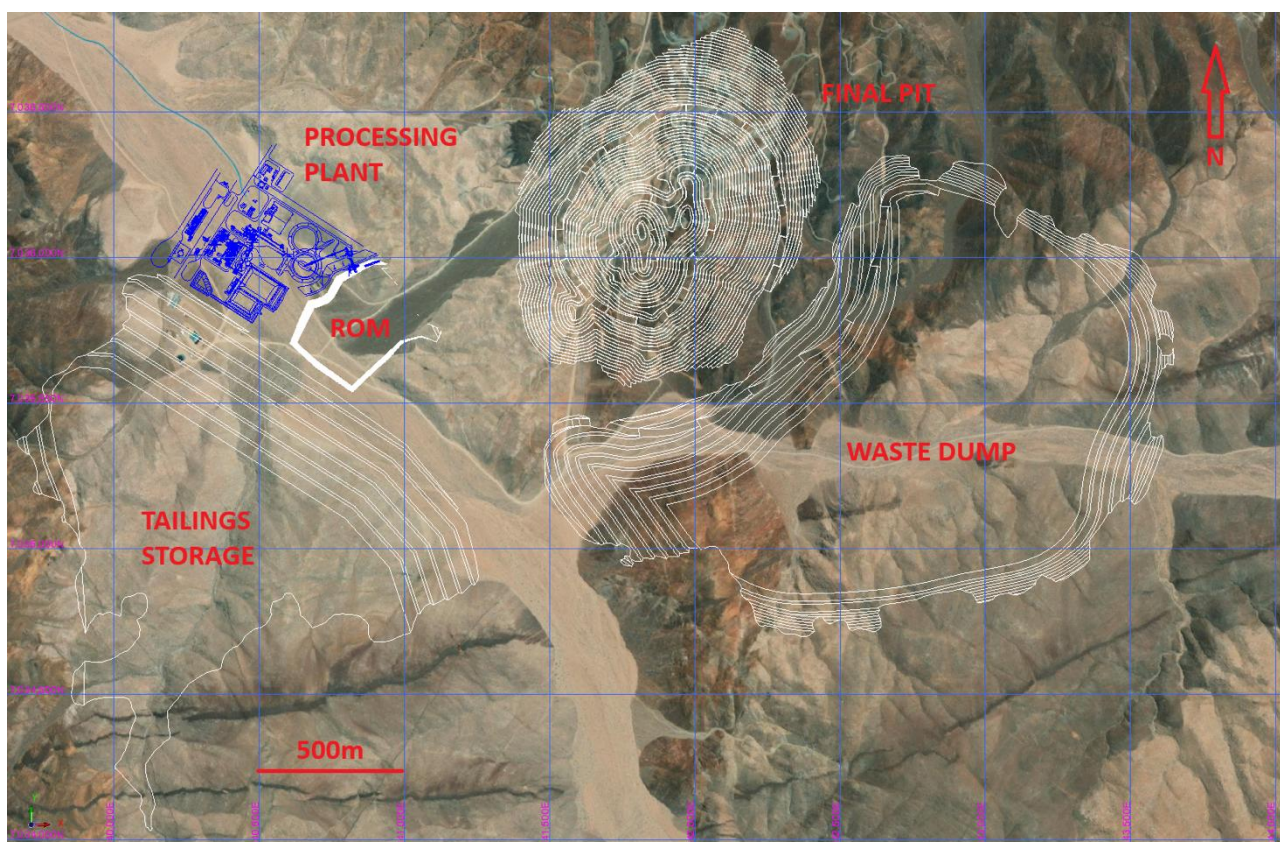
Figure 7 - El Zorro Site Layout
