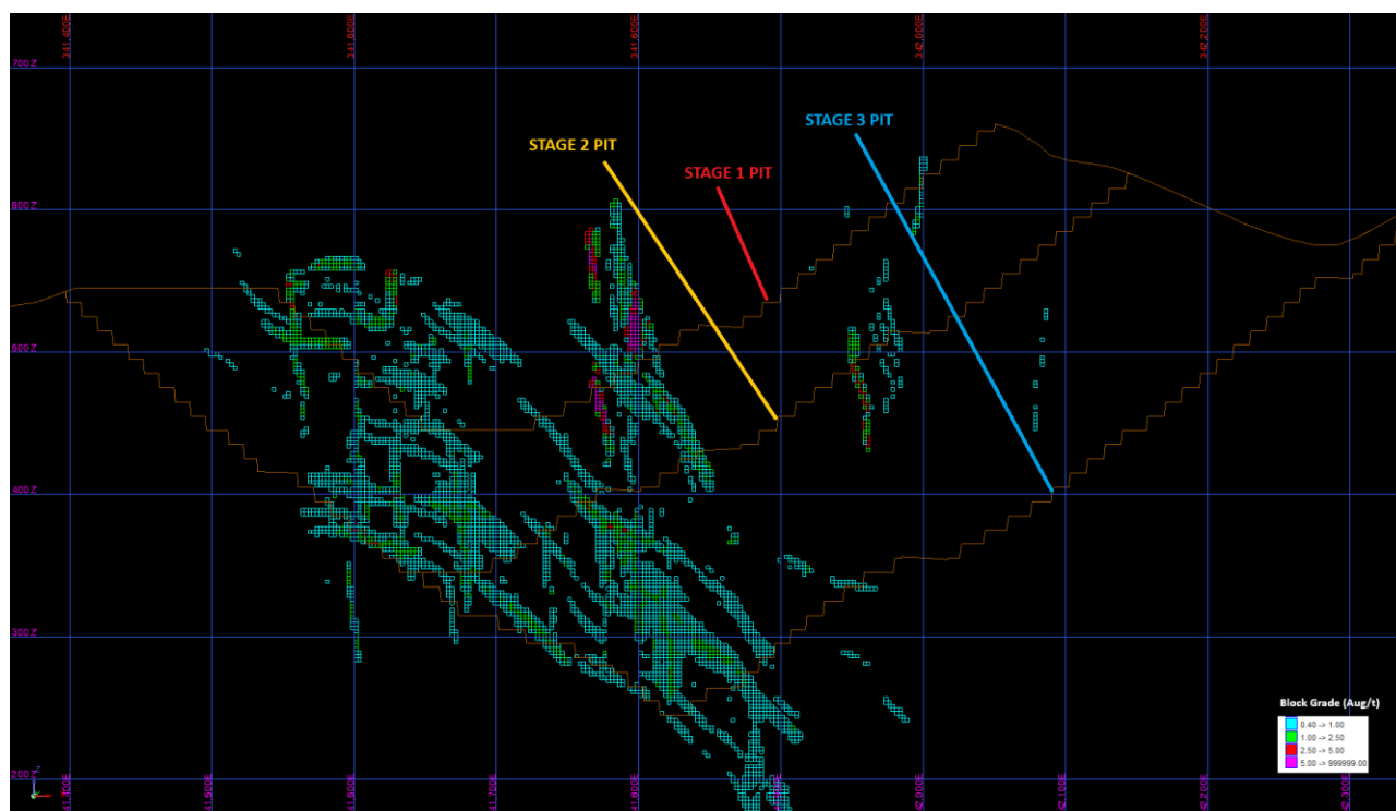
Figure 18 - Section 703600N - Looking North
