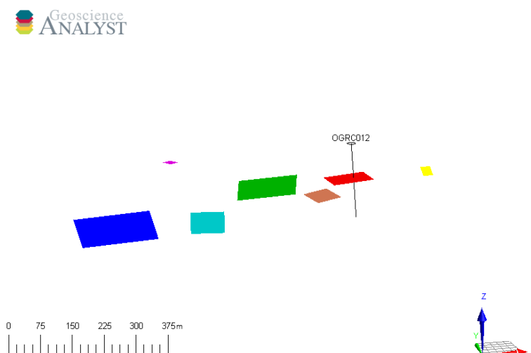
Figure 1. VT1 VTEM modelled 6 conductor plates, looking south (scale is in metres). OGRC012 tested the most accessible conductor.
