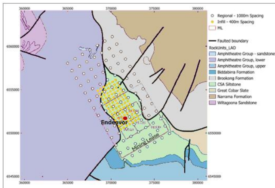
Figure 1. Design coverage of ANT survey (geological map after NSW Geological Survey)
